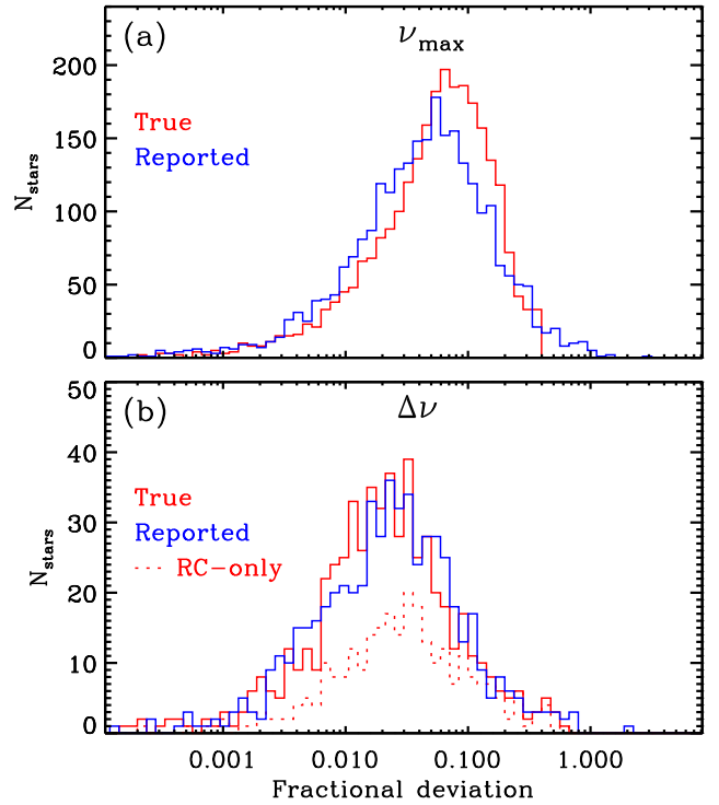
Figure 7. Deviations of TESS results for both \nu_{\max} and \Delta\nu are shown in panels (a) and (b), respectively. ‘True’ deviations are |\text{‘TESS’} - \text{‘Kepler’}| / \text{‘Kepler’} . ‘Reported’ deviations are random extracts from N(0, \sigma_{\text{TESS}} / \text{‘TESS’}) distributions.
