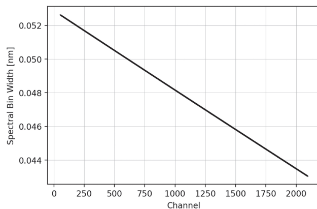
Fig. 6. Spectral bin width versus the CCD channel number for the UV spectrometer.
