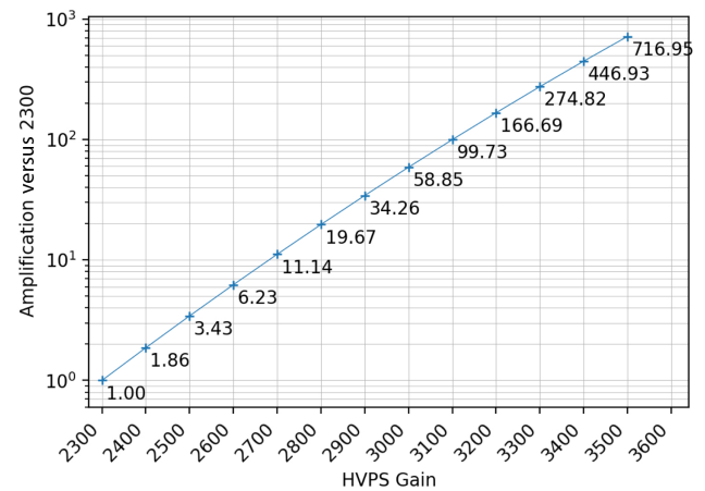
Fig. 15. Amplification factor relative to 2300 gain for various high voltage power supply (HVPS) gain settings for the intensifier used in the GOR spectrometer. The signals in the usable regions of the GOR regions were summed and ratioed to the sum of the signal collected with 2300 gain.
