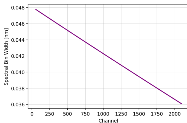
Fig. 7. Spectral bin width versus the CCD channel number for the VIO spectrometer.
