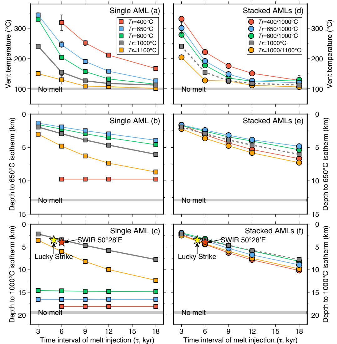
Figure 6. Key model outputs of simulations that vary the temperature of the host rock upon melt emplacement ( Tr ). See legend for the corresponding Tr values. Simulations with a given Tr have time intervals of melt injection varying from \tau = 3, 6, 9, 12 , to 18 kyr. The axial melt lens (AML) dimension is set to W_{AML} = 4 km and H_{AML} = 0.2 km in total. Hydrothermal domains are confined above Z_{H0} = 3 km with a permeability of k = 10^{-15} \text{ m}^2 . (a)–(c) Single AML emplacement. (d)–(f) Two stacked half-thick AMLs emplacements.
