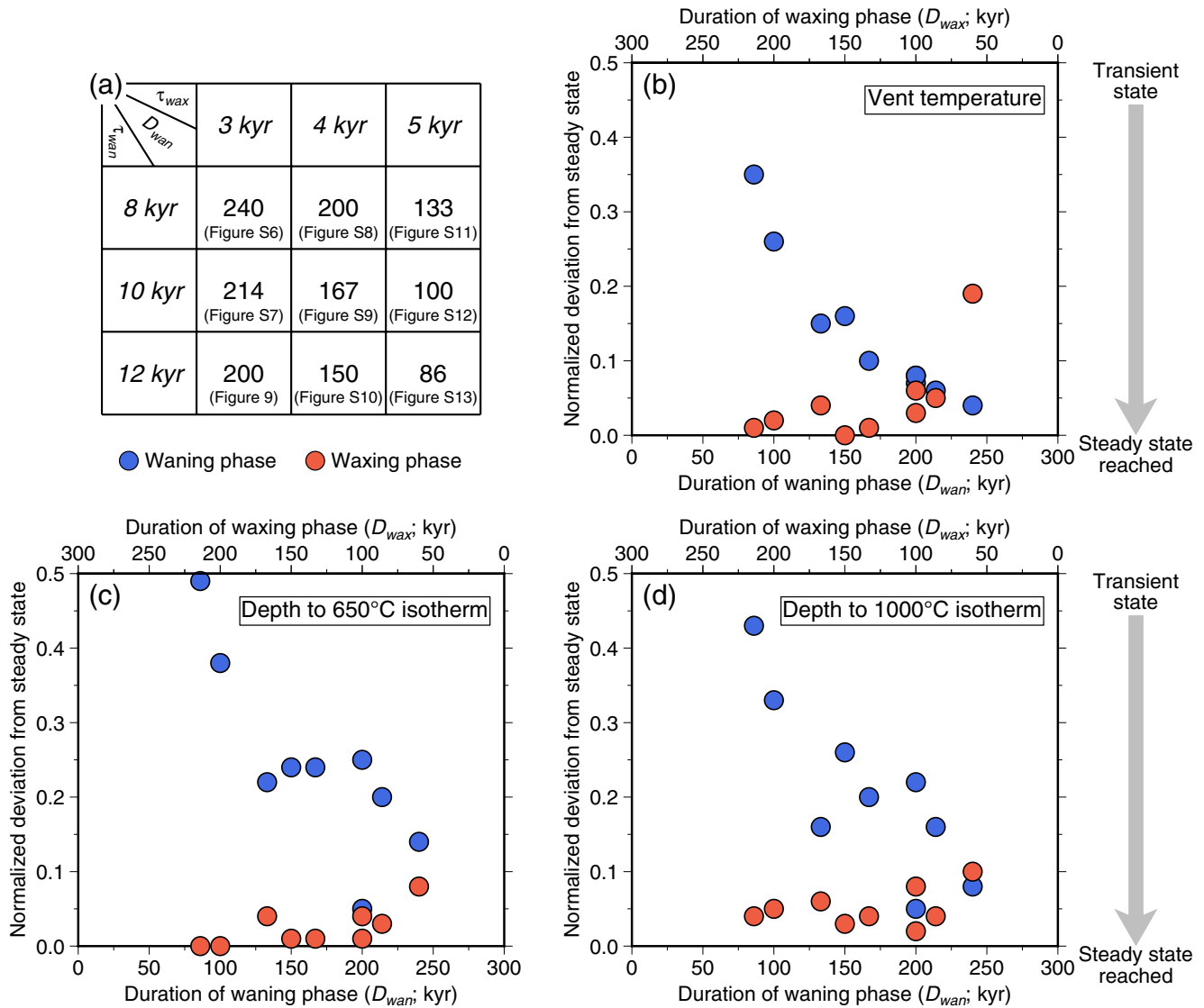
Figure 8. (a) 3×3 matrix of configurations of \tau_{wax} = 3, 4 , and 5 kyr and \tau_{wan} = 8, 10 , and 12 kyr. D_{wan} and D_{wax} are calculated by combining Equations 6 and 7. (b)–(d) Normalized deviations of vent temperature, and depths to the 650°C and 1,000°C isotherms, calculated by differences between values at the end of waxing (or waning) phases and at the steady state of the control simulation with \tau = \tau_{wax} (or \tau = \tau_{wan} ), which are normalized by the difference between two control simulations. \tau_{wax} : time interval of melt injections during waxing phases. \tau_{wan} : time interval of melt injections during waning phases. D_{wax} : duration of a waxing phase. D_{wan} : duration of a waning phase.
