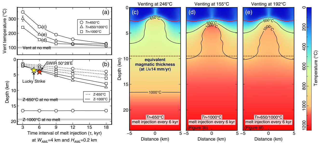
Figure 5. Simulations varying the temperature of the host rock upon melt emplacement: T_r = 650^\circ\text{C} , T_r = 1,000^\circ\text{C} , and T_r = 650/1,000^\circ\text{C} (half of the melt emplaced at T_r = 650^\circ\text{C} , and the other half at T_r = 1,000^\circ\text{C} ). See legend for symbols. Simulations with a given T_r have time intervals of melt injection varying from \tau = 3, 6, 9, 12 – 18 kyr. The AML dimension is set to W_{\text{AML}} = 4 km and H_{\text{AML}} = 0.2 km in total. Hydrothermal domains are confined above Z_{H_0} = 3 km with a permeability of k = 10^{-15} \text{ m}^2 . (a) Maximum vent temperatures in stationary states. Thick gray line represents the no-melt simulation (Figure 3f). (b) Depths to the 650^\circ\text{C} (dashed lines) and 1,000^\circ\text{C} (solid lines) isotherms. Red and yellow stars represent the depths to the mush zones of the SWIR 50°28'E and the Lucky Strike. (c)–(e) Snapshots of stationary-state thermal regimes for three selected T_r at \tau = 6 kyr. Equivalent magmatic thickness is shown for the SWIR spreading rate of 14 mm/yr. See Figure S4 in Supporting Information S1 for snapshots of \tau = 3, 9, 12 , and 18 kyr.
