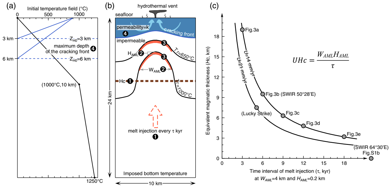
Figure 2. (a) Initial temperature field and the setting of the maximum depth of the cracking front ( Z_{H0} ). (b) Cartoon of the thermal model setup, modified from Fan et al. (2021). Numerical labels correspond to the four groups of simulations. (c) Equivalent magmatic thickness ( H_c ) versus time interval of melt injection ( \tau ) at W_{AML} = 4 km and H_{AML} = 0.2 km, according to Equation 5. W_{AML} , width of AML; H_{AML} , thickness of AML; T_r , temperature of host rock upon melt emplacement; U , full spreading rate.
