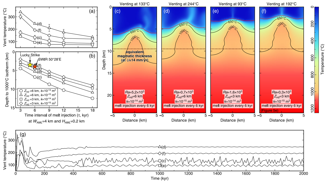
Figure 7. Simulations of four combinations of the maximum hydrothermal domain depths ( Z_{H0} = 3 and 6 km) and permeabilities ( k = 10^{-15} and 10^{-14} m 2 ). See legend for symbols. Each combination has time intervals of melt injection varying from \tau = 3, 6, 9, 12 , to 18 kyr. The AML dimension is set to W_{AML} = 4 km and H_{AML} = 0.2 km in total, emplaced beneath Tr = 650/1,000^\circ\text{C} . (a) Maximum vent temperatures in stationary states. (b) Depths to the 1,000^\circ\text{C} isotherms. (c)–(f) Snapshots of stationary-state thermal regimes for four combinations at \tau = 6 kyr. The equivalent magmatic thickness is calculated for the SWIR spreading rate of 14 mm/yr. (g) Maximum vent temperatures throughout the first 2,000 kyr of simulations for four combinations. Ra : Rayleigh number of hydrothermal convection system. See Figure S5 in Supporting Information S1 for snapshots of \tau = 3, 9, 12 , and 18 kyr.
