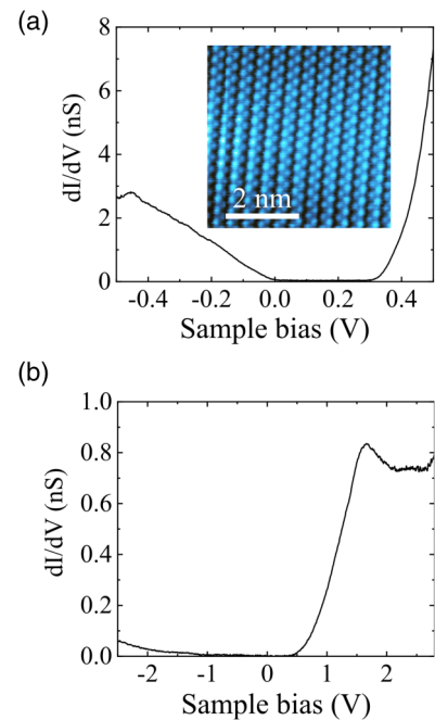
FIG. 4. (a) Experimental dI/dV spectrum of a bulk BP sample. The inset shows an STM image with atomic resolution of the area where the spectrum was measured (sample bias 0.2 V, tunneling current setpoint 600 pA), and (b) dI/dV spectrum measured over a larger sample bias range.
