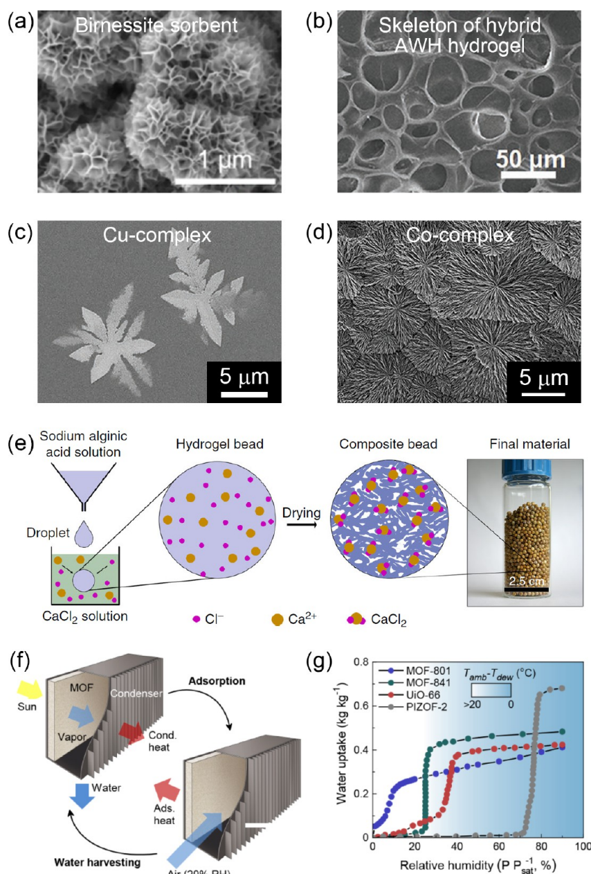
Figure 7. Examples of common desiccant materials, composites and MOFs adopted in passive indirect AWH systems. (a) SEM image of layered birnessite MnO 2 structure. [Reproduced with permission from ref 165. Copyright 2019, American Chemical Society, Washington, DC.] (b) SEM image of hybrid skeleton-shaped hydrogel consisting of hygroscopic polymer and hydrophilic gel. [Reproduced with permission from ref 167. Copyright 2019, Wiley–VCH Verlag GmbH & Co. KGaA, Weinheim, Germany.] (c) SEM image of Cu-complex. [Reproduced with permission from ref 168. Copyright 2020, Wiley–VCH GmbH.] (d) SEM image of Co-based super hygroscopic complex. [Reproduced with permission from ref 169. Copyright 2021, Wiley–VCH GmbH.] (e) Schematic of the production process for the composite beads consisting of alginate-derived matrix and embedded calcium chloride. [Reproduced with permission from ref 175. Copyright 2018, Springer Nature, Limited.] (f) Schematic of MOF-801-based AWH system prototype. (g) Water adsorption isotherms for several Zr-based MOFs, including MOF-801. [Reproduced with permission from ref 185. Copyright 2017, American Association for the Advancement of Science.]
