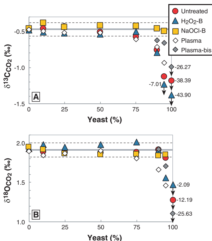
Fig 2. \delta^{13}\text{C}_{\text{CO}_2} (A) and \delta^{18}\text{O}_{\text{CO}_2} (B) values of the dolomite mixture samples as a function of the yeast proportion (%). The gray lines represent the average isotope compositions of pure dolomite (INYO) and the dotted lines indicate a \pm 0.1 ‰ range. The errors are comprised within symbols.
