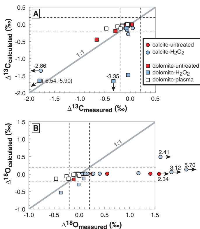
Fig 6. Comparison between the isotope shifts measured for mixture samples and those calculated assuming a \text{CO}_2 contribution from yeast. The gray line represents the 1:1 line where the points should align in case of a \text{CO}_2 contribution from yeast.
