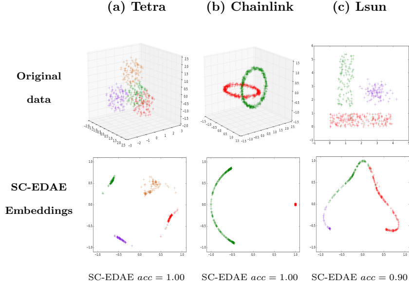
Figure 2: Visualization of the SC-EDAE embeddings on Tetra , Chainlink and Lsun datasets. The two first components of B (Alg.1, step (c)) gives a visualization of the datapoints separability with the SC-EDAE method. Colors indicate the predicted labels.
