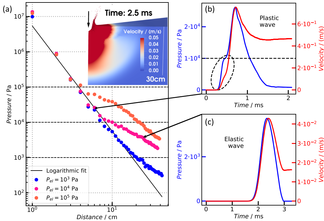
Figure 2. Evidence of an elastic and plastic regimes. (a) The maximum modeled pressure recorded with distance for three different values of P_{el} . In inset, a snapshot of a HOSS simulation of the 0.98 km/s shot, showing the amplitude of the velocity and the ejected sand elements 2.5 ms after the impact. (b) Waveform in an area where P exceeds P_{el} = 10^4 Pa. The dashed circle indicates the elastic precursor followed by the plastic wave. (c) Waveform in an area further away from the impact with only an elastic wave. P_{el} appears to be an important parameter controlling the transition between these two regimes.
