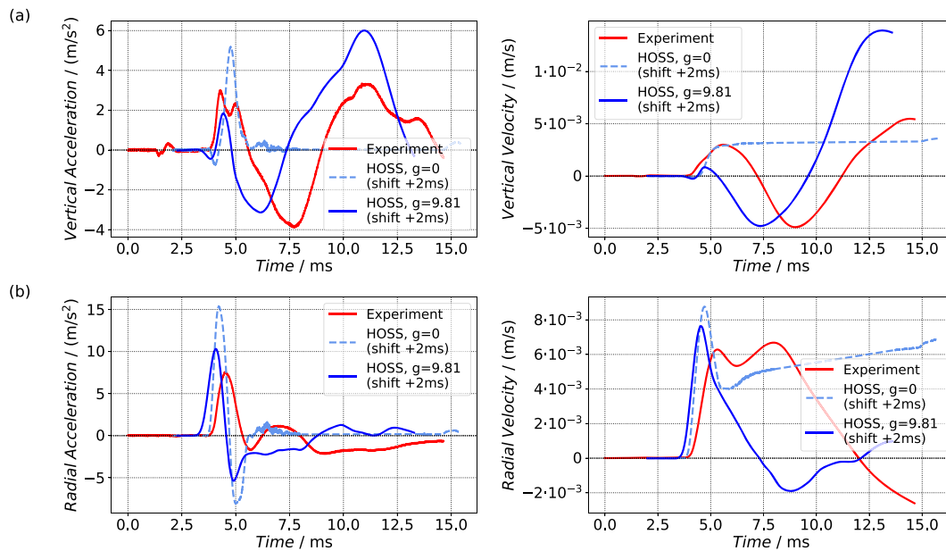
Figure 4. Compared numerical and experimental (a) vertical and (b) radial signals for the 0.98 km/s impact velocity shot. Both accelerations and velocities are shown for the sensor 30 cm radially away from the impact point. The solid blue line and the dashed light-blue line correspond to simulations performed with and without earth gravity, respectively. Note that modeled signals have been shifted in time to obtain a better match (see text for details).
