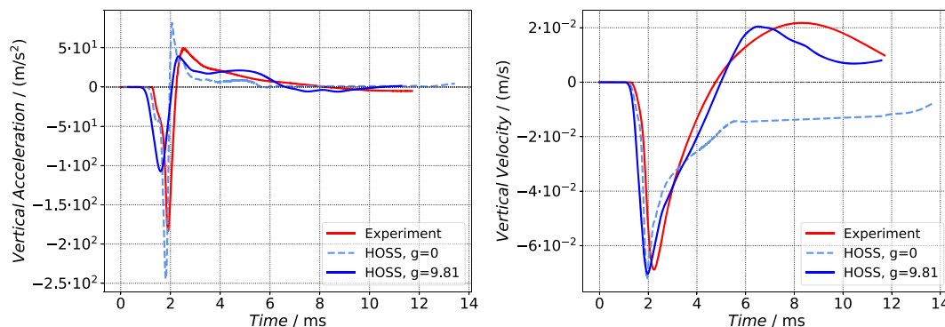
Figure 3. Compared numerical and experimental vertical acceleration (left) and velocity (right) signals for the 0.98 km/s impact velocity shot, recorded at a sensor 21 cm directly below the impact point. The solid blue line and the dashed light-blue line correspond to simulations performed with and without earth gravity, respectively. The simulation better matches the experiment when gravity is considered.
