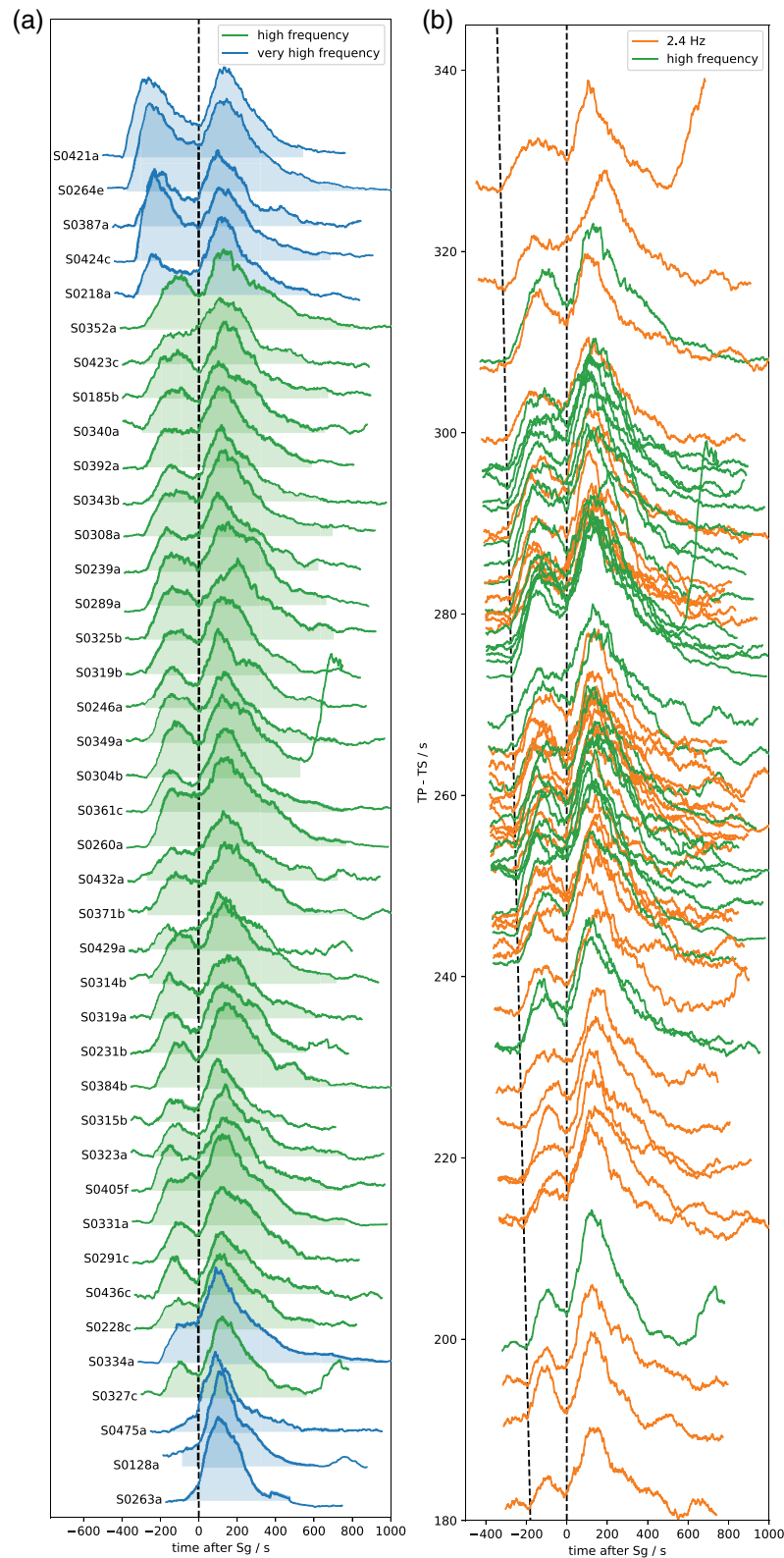
Figure 6. (a) Normalized 2.4 Hz vertical component envelopes for all quality B HF and VF events with regular spacing, ordered by distance. (b) Same for all quality B 2.4 and HF events with vertical alignment proportional to the relative arrival time of the two phases ( P_g and S_g ). Note that different SNRs cause the impression of different amplitudes and some events are followed by unrelated noise signals (e.g., S0304b and S0327c). Events are aligned on arrival time of the S_g phase, the filled range in (a) indicates the time window of the event as picked in the catalog. HF, high frequency; VF, very high frequency; SNR, signal-to-noise ratio.
