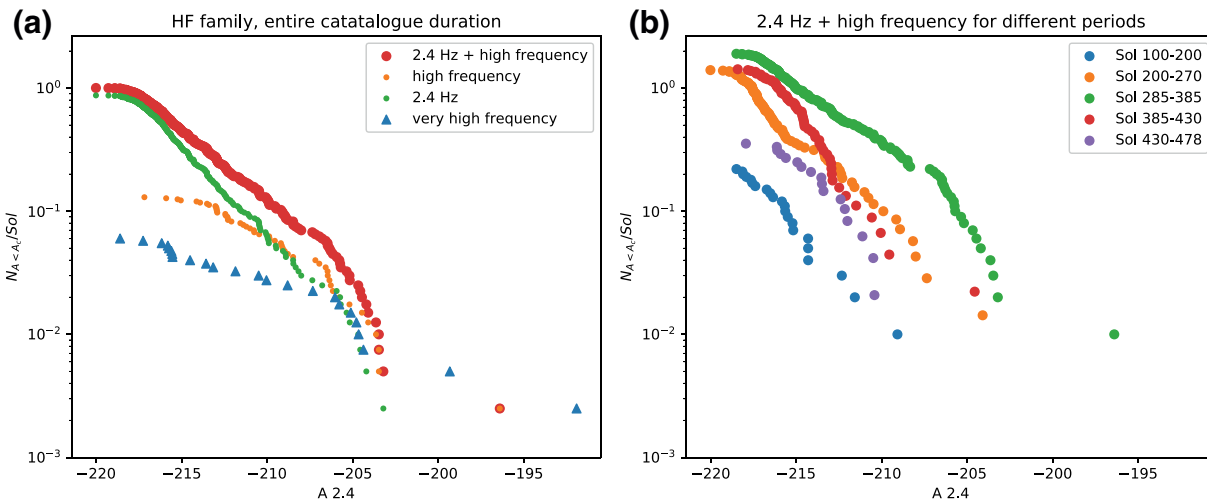
Figure 9. (a) Cumulative size-frequency distribution normalized to one sol for the different event types. (b) Same for 2.4 Hz and HF events combined for several time windows in the mission. The number of events per sol varies by more than an order of magnitude, which is significantly more than the variation in the noise level and length of the quiet evening windows. HF, high frequency.
