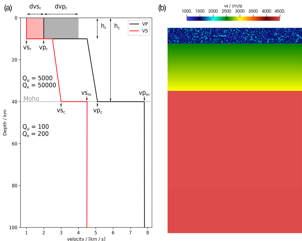
Figure 12. (a) Reference model and parametrization from which all other models are created by perturbing single parameters. (b) Section of one random realization of the reference model.
