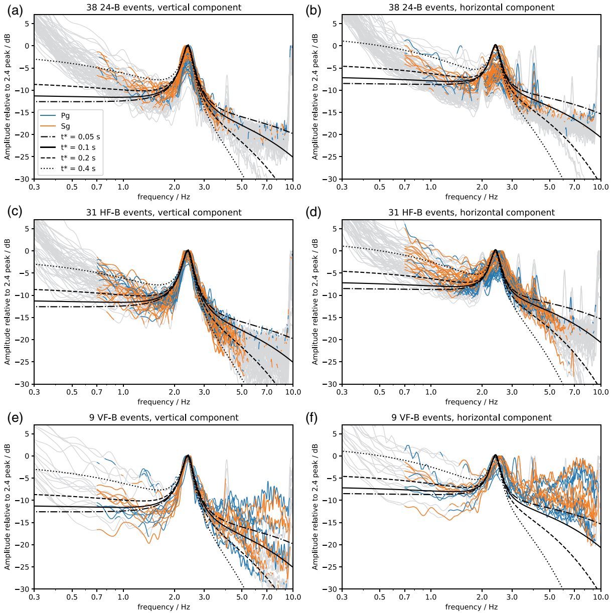
Figure 7. Displacement spectra for quality B 2.4 Hz (a)–(b), HF (c)–(d) and VF (e)–(f) events for vertical (a, c, e) and horizontal components (b, d, f). For frequencies above 0.7 Hz, the lines are colored where the SNR is above a value of 2. Black lines indicate expected spectra assuming a flat source spectrum modulated by a resonance (amplification factors 30 on the vertical and 10 on the horizontal) and frequency independent attenuation with different quality factors. The difference in amplitude at frequencies about 5 Hz is the main discriminant between the HF and VF event classes. HF, high frequency; VF, very high frequency.
