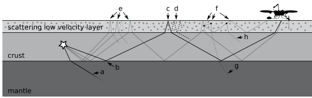
Figure 11. Ray paths that contribute to the two broad arrivals in the numerical model. Specific effects indicated by arrows are detailed in the text.
