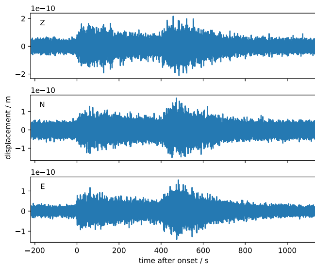
Figure 3. Three component displacement seismogram for S0421a filtered in the frequency range 0.5–7 Hz. The telltale sign of an HF event are the two distinct energy pulses that are separated by up to several minutes, both of which have an emergent onset and a long coda. HF, high frequency.
