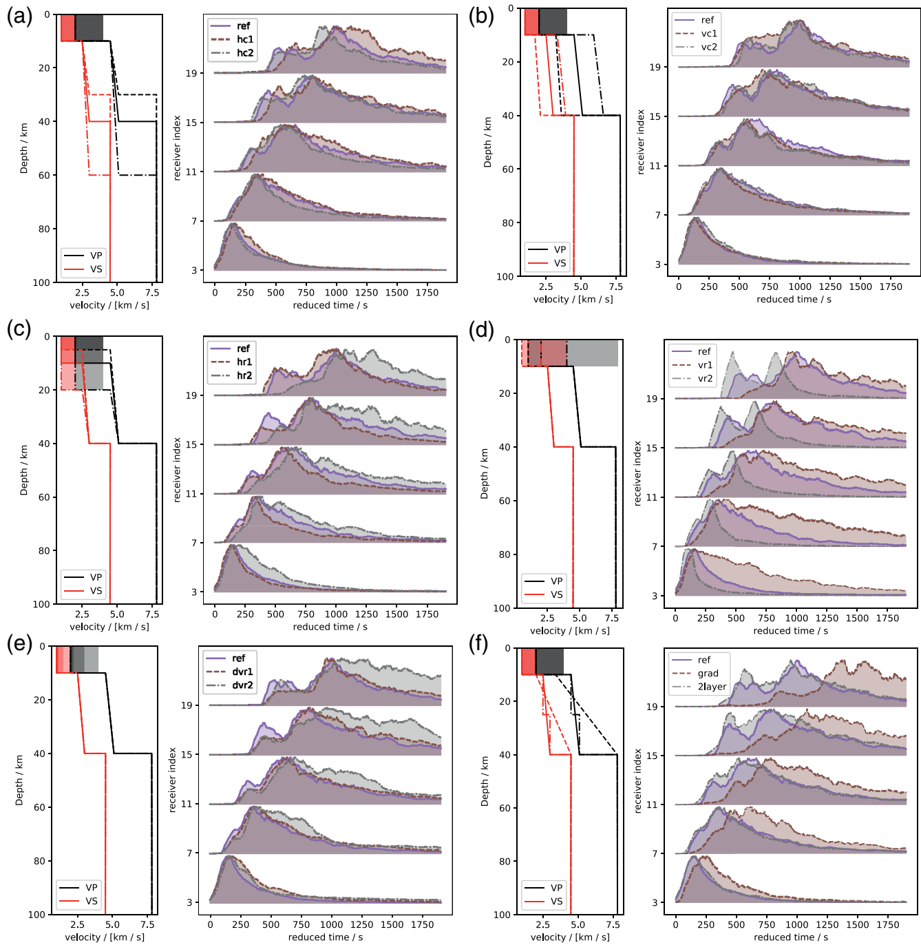
Figure 14. Sensitivity analysis for synthetic envelopes to changes in (a) crustal thickness and (b) velocities, (c) shallow layer thickness, (d) velocities and (e) scattering strength. (f) shows a model without a first order discontinuity at the moho and one with two crustal layers. Receivers are placed such that the estimated guided phase traveltimes based on the fastest crustal velocities are similar and hence the envelopes more directly comparable in time.
