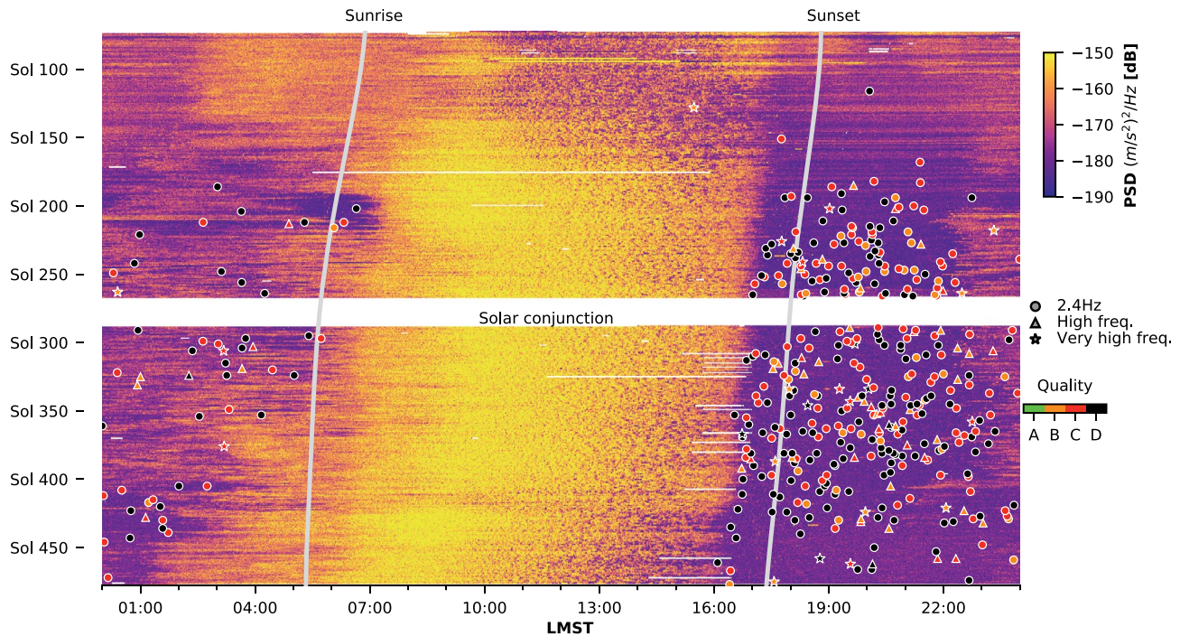
Figure 4. Evolution of the noise power spectral density (PSD) on the VBB vertical component in the 2.3–2.6 Hz frequency range (i.e., the resonance excited by events) since placement of the wind and thermal shield (WTS). For each sol, the figure shows the spectrogram as in Figure 1, but vertically constrained to the resonance as an indicator of the detection capability. The symbols indicate the distribution of the high-frequency events until 31 March 2020 (sol 478) and their signal quality as detailed in the text. The noise patterns correlate with the sunrise and sunset, indicated by the white lines. Solar conjunction prohibited data transfer from sol 268 to 288. VBB, very broad band.
