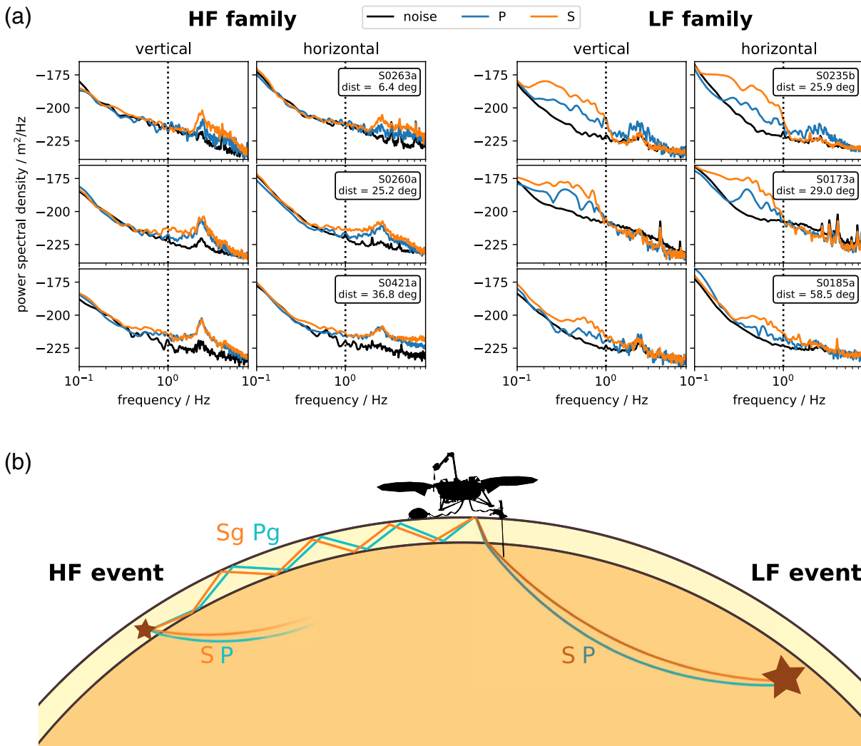
Figure 2. (a) Spectra of several events from the two event families: a clear separation based on the main energy content above or below 1 Hz. (b) Current interpretation of the two event families: similar relative traveltimes between the two main arrivals but very different frequency content can be explained by different source depth and propagation paths in the crust and upper mantle with different attenuation regimes. Figure modified from Giardini et al. (2020).
