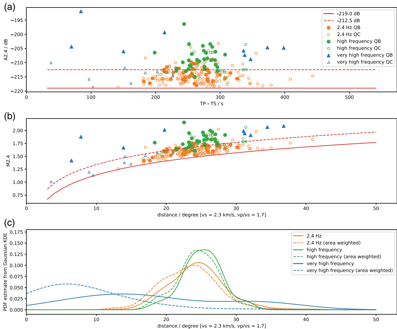
Figure 8. (a) Spectral amplitude measured on the 2.4 Hz resonance versus relative arrival times of Pg and Sg. The red solid line represents the detection thresholds during the quietest times of the mission and the red dashed line indicates the amplitude at which most events are visible outside the resonance. (b) Assuming seismic velocities, distances in degrees and Magnitudes can be assigned. (c) Kernel density estimation with distances weighted according to the corresponding surface area confirms that 2.4 Hz and HF events are clustered around a relative traveltime of 280 s, while VF events are more evenly distributed. HF, high frequency; VF, very high frequency.
