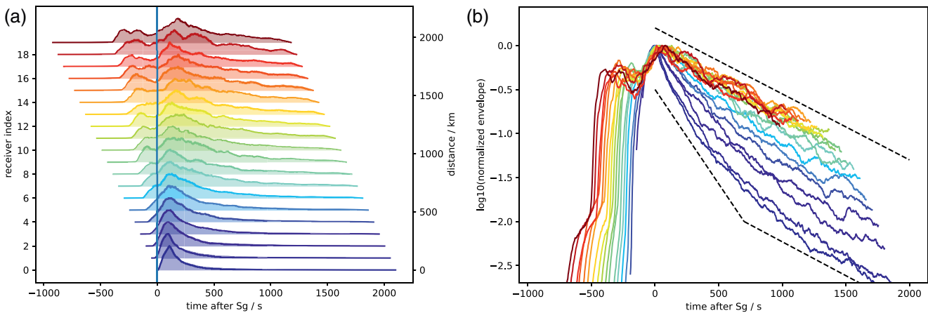
Figure 13. Envelopes of synthetic seismograms computed in the reference model with a source at 30 km depth, smoothed with a 100s boxcar window and aligned on the Sg-arrival time. The traces are aligned by epicentral distance in (a) as also indicated by the color. The logarithmic scaling in (b) highlights that at later times the coda-decay is independent of the distance. For closer events, the initial decay is faster though before it approaches the same value after several hundreds of seconds as indicated by the dashed lines. The mantle P-wave is also visible as a precursor at very small amplitude.
