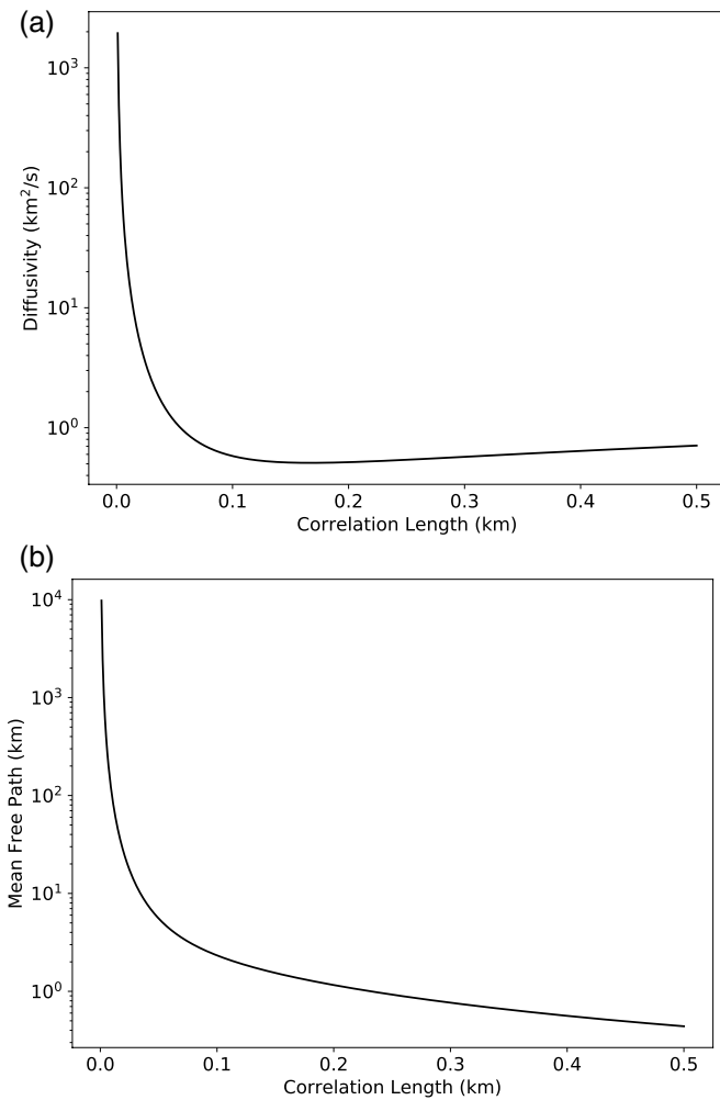
Figure 15. Estimate of the diffusivity (a) and the shear mean free path (b) for the heterogeneous models used in the numerical simulations, as a function of the correlation length.
