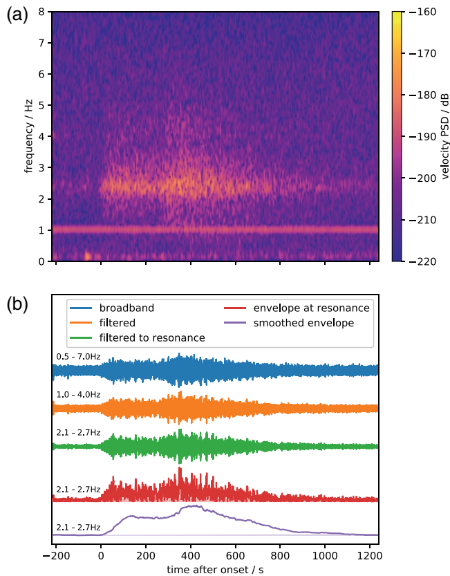
Figure 5. (a) Spectrogram of the VBB vertical component velocity for the quality B HF event S0260a. The monochromatic signal at 1 Hz is known as “tick noise” and caused by electronic crosstalk (Ceylan et al., 2020). (b) Broad-band signal (blue, orange, green) and envelope filtered in different frequency ranges (indicated on the left above each waveform). The purple envelope has been convolved with a 100 s boxcar window. This processing maintains the onset times and thus allows picking of the two main phases also for weaker events. VBB, very broad band.
