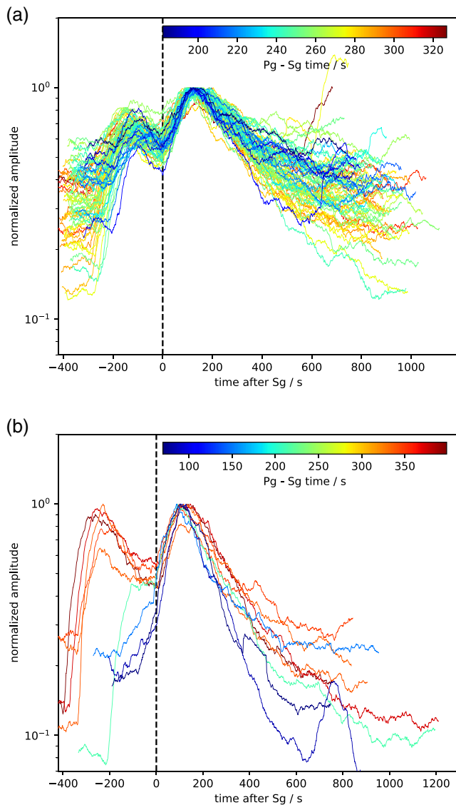
Figure 10. All quality B 2.4 Hz and HF events (a) as well as VF events (b) aligned on the Sg arrival and scaled to the same amplitude. The color of each line corresponds to the relative traveltime, note the different colorbars. The coda shape of the Sg phase has no significant systematic dependency on the distance for 2.4 Hz and HF events in contrast to the VF events. HF, high frequency; VF, very high frequency.
