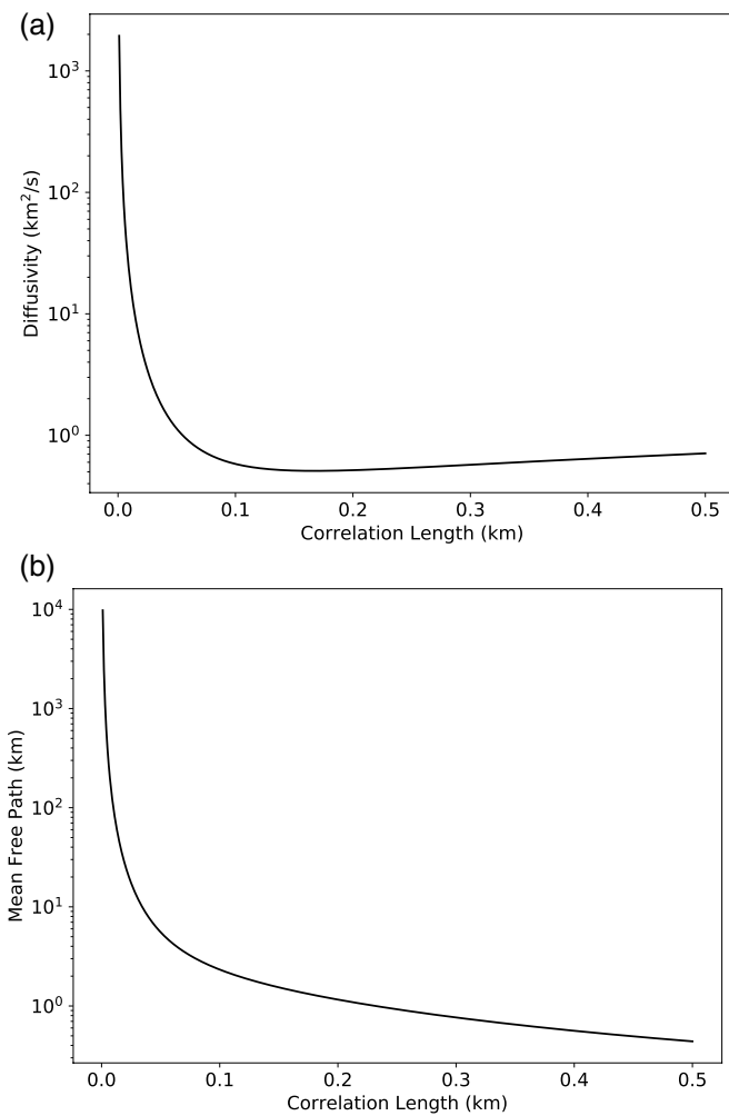
Figure 15. Estimate of the diffusivity (a) and the shear mean free path (b) for the heterogeneous models used in the numerical simulations, as a function of the correlation length.
