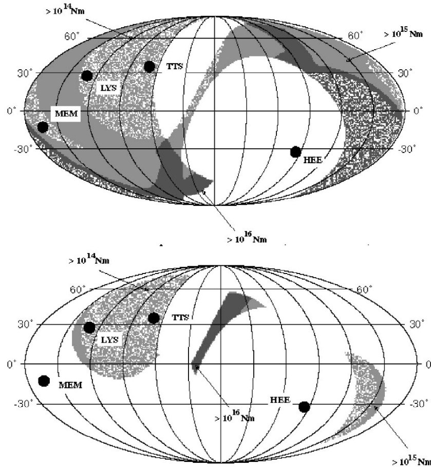
Figure 34a: (Top) Detection zone of P and S waves for one of the studied configuration in the former Netlander project (MEM, LYS, TTS and HEE are respectively Menomnia Fosae, Lycus Sulci, Tempe Terra South and Hellas East). The white zone on to the east of TTS corresponds to the joint shadow zone of MEM and HEE. Note that the detection efficiency is very high in the Tharsis area, where small quakes of seismic moment of 10^{14} Nm might be detected. (Bottom) Detection zone for a detection of a PKP wave in at least one station and of PandS waves in the three other stations. The success rate is 16%, leading to about 22 quakes detected during the two years of operation. Reprinted from Lognonné et al. (2000) with permission of Planetary Space Science.
