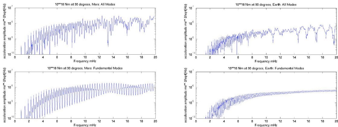
Figure 35a-b: Acceleration amplitude spectrum for a quake with strike, deep, rake angles of 45°, 45°, 45° and a seismic moment of 10^{18} Nm. Azimuth is 20° and the epicentral distance is 90°. The depth of the event is 30 km. Spectrum for Mars are shown on (a). Those for the Earth are on (b). At 5 mHz, the amplitudes exceed 1 ng Hz -1/2 and are a factor 4 greater than those observed on the Earth. Note that below 10 mHz, the fundamental modes are associated to most of the signal.
