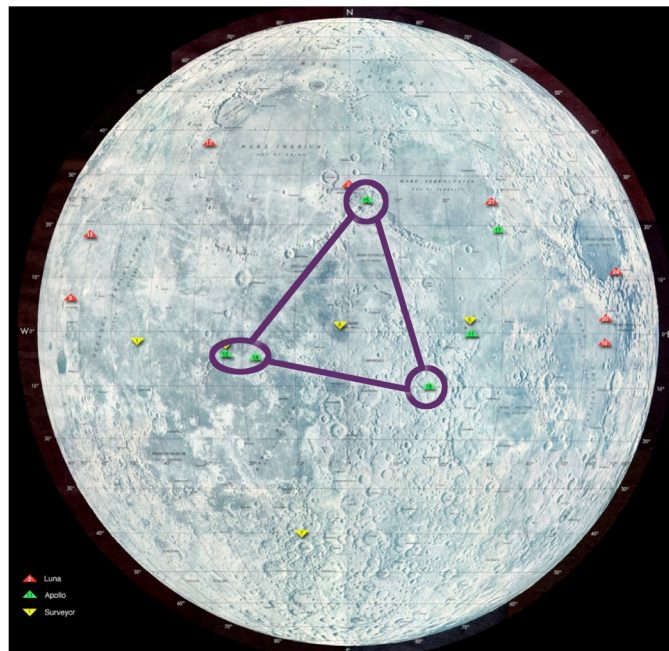
Figure 2: Configuration of the Apollo Seismic Network, A12 is in the Oceanus Procellarum area at 3.01 S, 23.42 W, A14 is located near the crater Fra Mauro at 3.64 S, 17.47 W, A15 is at the foot of the Apennine mountain range at 26.13 N, 3.63 E and A16 is just north of the crater Dolland at 8.97 S, 15.50 E. Note that all stations were on the near side, leading core seismic studies almost impossible. Base map credit NASA.
