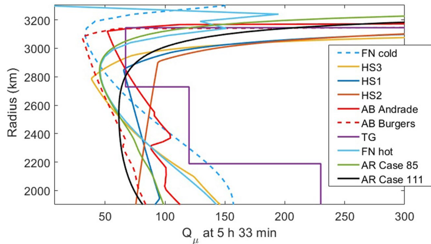
Figure 3. Q_{\mu} profile at the main Phobos tide period (5.55 hr). Since the tidal bulk Q_{2200} is strongly constrained through the secular acceleration of Phobos, all models show a similar Q_{\mu} profile at this frequency.
