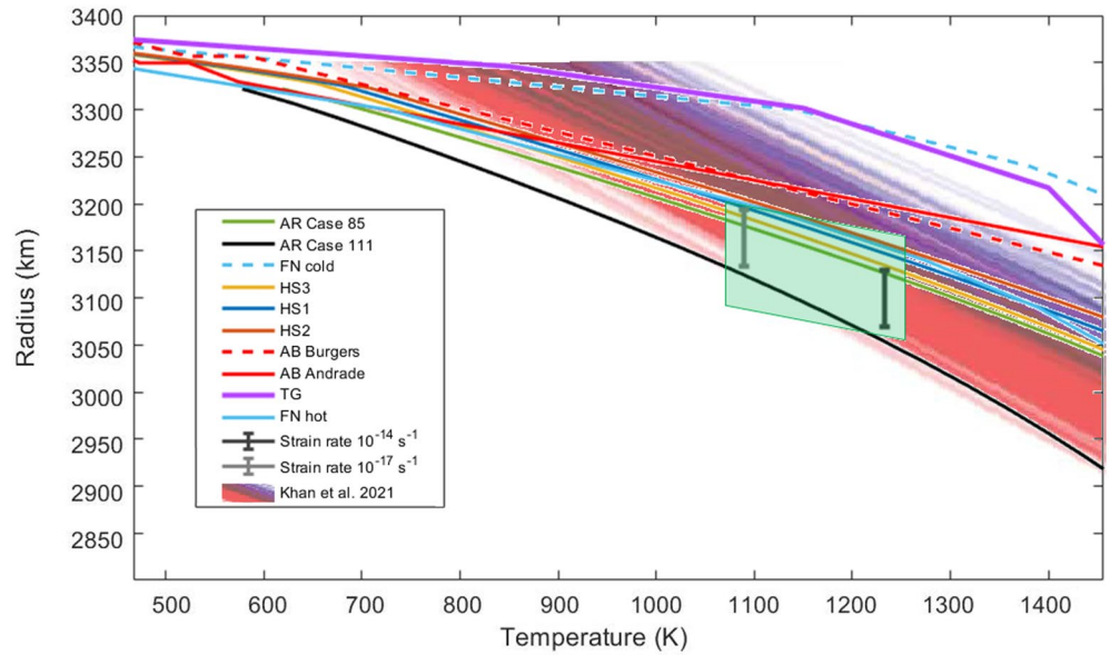
Figure 6. Constraints from the elastic thickness on the temperature profiles, for strain rates between 10^{-14}\text{s}^{-1} and 10^{-17}\text{s}^{-1} based on Grott and Breuer (2008) and Plesa et al. (2018) and comparison with the upper mantle inversions from seismic waves from Khan et al. (2021). The green area delimited by the vertical black segments highlights the possible temperatures at the base of the elastic layer from thermal modeling (e.g., Plesa et al., 2018) that are consistent with the observed lithospheric flexure from Broquet et al. (2020) and Broquet et al. (2021). The red band from Khan et al. (2021) are models with a thermal lithosphere thickness between 400 and 500 km from geophysical inversions, while the blue band are between 500 and 600 km from seismic inversions. Hotter models do not fit the inferred elastic thickness. Colder models with a higher average elastic thickness are capable of fitting the polar elastic thickness.
