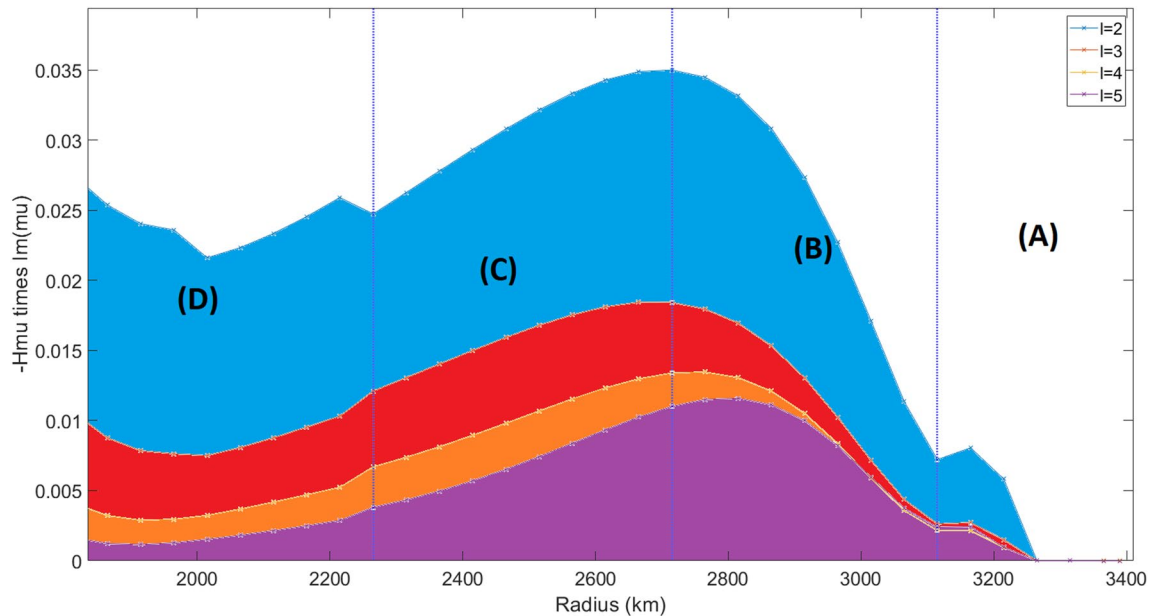
Figure 4. Sensitivity parameter H_\mu multiplied by the imaginary part of the shear modulus \text{Im}(\mu) (right-hand side term in Equation 20) in the Martian model for the FN hot model, for degree 2 up to 5. The surface area below each curve represents the dissipation in each layer of the Martian interior that contributes to the bulk tidal dissipation rate k_\ell/Q_\ell . Mantle subdivisions are indicated with blue lines (details in text). This takes into account the actual value of Q_\mu in the mantle to show that for this model, dissipation is actually stronger in the upper layer of the lower mantle (C area) due to its lower Q_\mu compared to the lower layer of the lower mantle (D area), and it is clearly visible that the lithosphere has a very limited impact and almost none for the crust.
