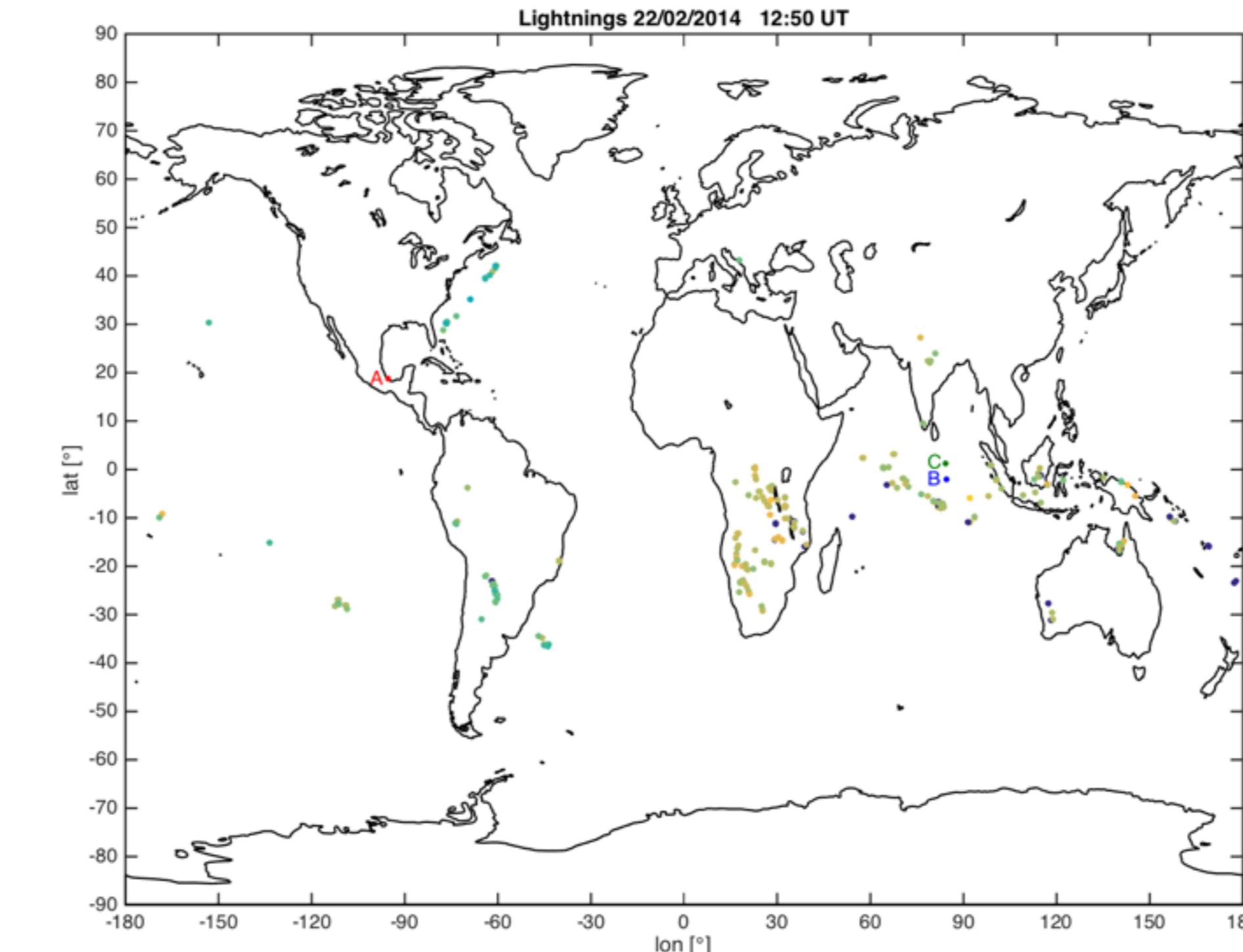
Figure 5: Map of lightning strokes occurred on 22 February 2014 during the minute starting at 12:50 UT. Satellites B and C were flying above the Indian Ocean. The strongest lightning occurred at 12:50:22.18 in that region, most likely producing the large signal seen in Figure 3.
