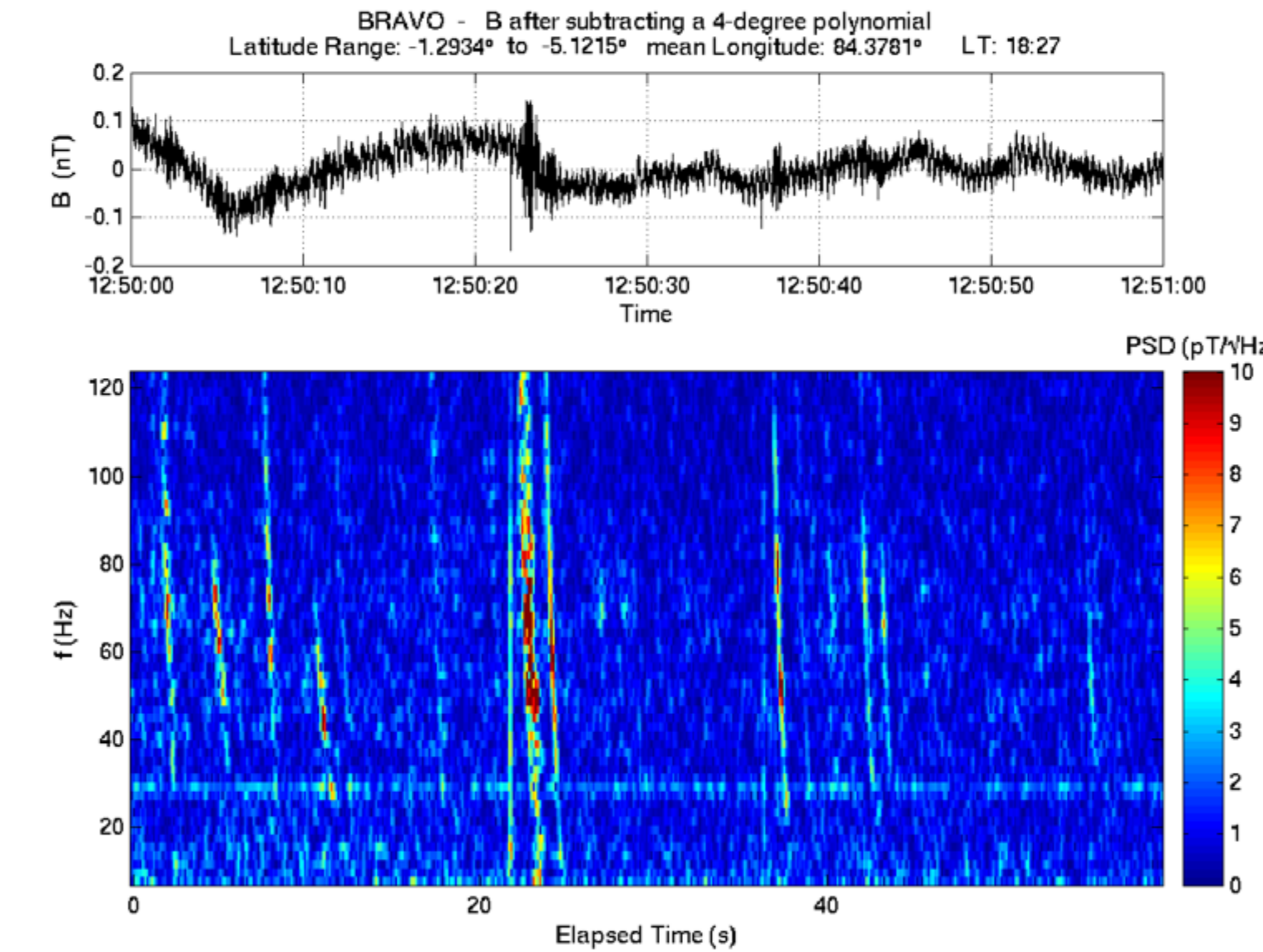
Figure 3: Electromagnetic signals detected on 22/2/2015 during the minute starting at 12:50 UT. Both Swarm B and C detections are simultaneous (397 km distance).
