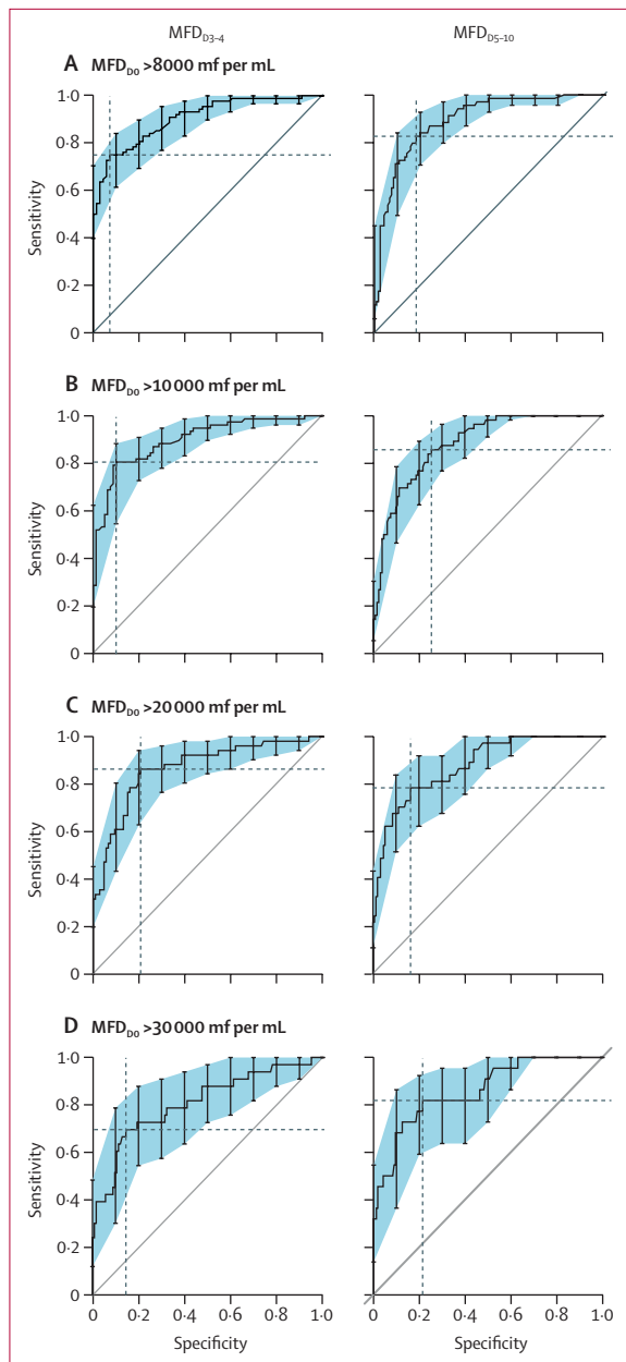
Figure 1 ROC curves for determining Loa loa MFD 00 from L. loa MFD D3-4 or L. loa MFD D5-10 (A) ROC curves for determining L. loa MFD 00 higher than 8000 mf per mL. (B) ROC curves for determining L. loa MFD 00 higher than 10000 mf per mL. (C) ROC curves for determining L. loa MFD 00 higher than 20000 mf per mL. (D) ROC curves for determining L. loa MFD 00 higher than 30000 mf per mL. The curves are determined from L. loa MFD D3-4 (first column) or L. loa MFD D5-10 (second column). The intersection of the dotted lines represents the best sensitivity-specificity pairing according to Youden's method. ROC=receiver operating characteristic. mf per mL= L. loa microfilariae per mL of blood. MFD= Loa loa microfilariae density. MFD 00 =MFD before ivermectin treatment. MFD D3-4 =MFD at day 3–4 after treatment. MFD D5-10 =MFD at day 5–10 after treatment.
