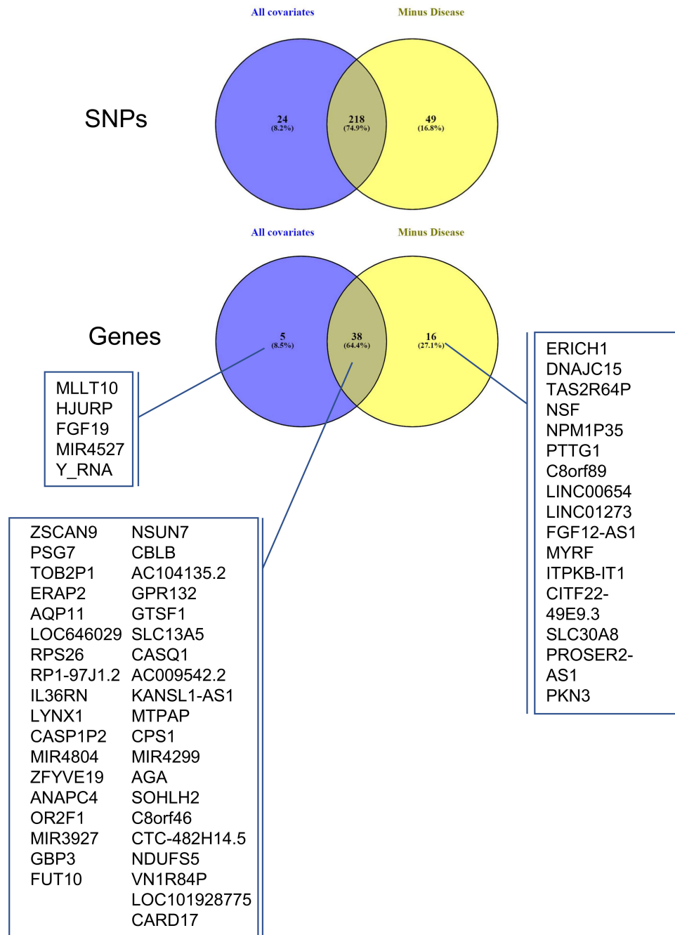
Figure 5. Overlap between cis-QTL datasets ALL COVARIATES and MINUS DISEASE. Venn diagrams showing the overlap between the eSNPs and eGenes identified as statistically significant (FDR ≤ 0.05) in ALL COVARIATES (blue) and MINUS DISEASE (yellow).
