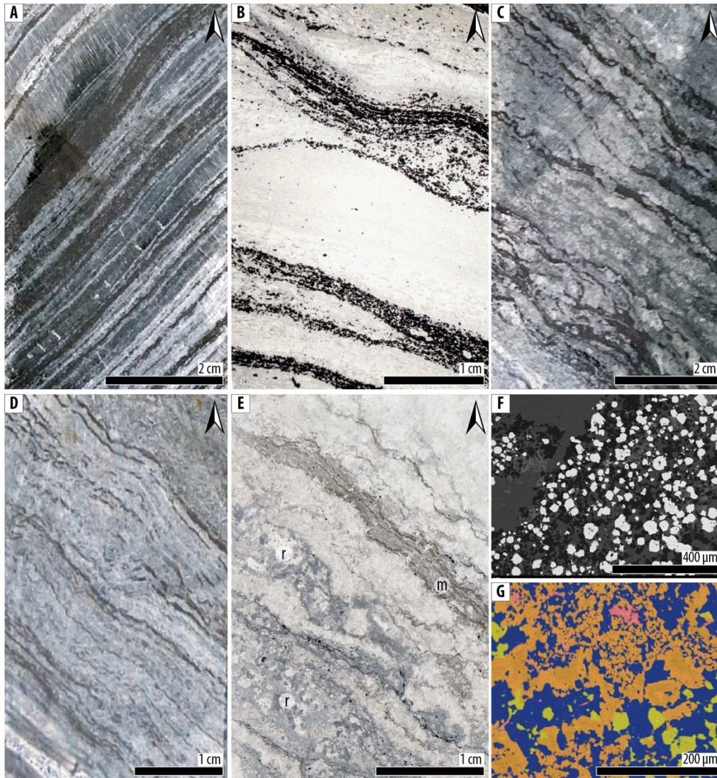
61 62 Fig. S3. Carbonate facies of the Carajás Formation. Arrows point to the stratigraphic top. A. 63 Sample FD55-521.60. Fine laminations (mm to cm scale) of iron-bearing minerals (mainly 64 magnetite) and carbonate layers. B. Sample FD55-521.12. Thin section in reflected light showing 65 wavy laminations underlined by magnetite grains and carbonates. C. Sample FD55-518.50. 66 Carbonate with irregular, crinkled magnetite laminations and pinching out geometries. D. Sample 67 FD55-522.56. Carbonate with very fine, crinkled lamination underlined by very fine (mm thick) 68 magnetite layers. E. Sample FD55-520.06. Thin section in reflected light showing a microbial mat 69 (m) within carbonate displaying a clotted micritic texture. Some areas show recrystallized (r) 70 textures. F. Sample FD55-514.57. Electron backscattered image showing diagenetic framboidal 71 pyrite (bright white) minerals within a carbonate matrix. G. Sample FD55-514.57. EDS electron 72 image showing Si, Ca and Fe-rich mineral phases.
