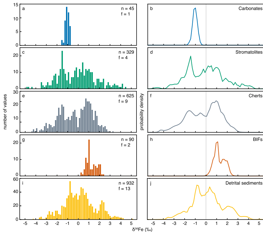
Fig. 5. Pyrite \delta^{56}\text{Fe} distributions in carbonates (a, b), stromatolites (c, d), cherts (e, f), BIFs (g, h), and detrital sediments (i, j). The distributions are shown as histograms (a, c, e, g, i) and the corresponding probability density plots (b, d, f, h, j). The numbers of values (n) and geological formations (f) from which pyrite originates are indicated on the histograms. The vertical grey bar on the right panels represents a \delta^{56}\text{Fe} value of 0‰ and is drawn to facilitate comparison between plots. Stromatolite distribution includes data measured in pyrite grains hosted in stromatolitic carbonate, stromatolite and stromatolitic chert (see data_compilation.xlsx in supplementary materials). Similarly, the chert distribution includes data measured in pyrite hosted in (black or white) chert, chert with barite, amphibole-rich cherts. The detrital sediment distribution includes data measured in pyrite hosted in (green, grey, black, calcareous or tuffaceous) mudstone, black shale, diamictite, (siliceous, calcareous or tuffaceous) sandstone, quartz-pyrite pebble, carbonaceous shale, carbonate laminated siltstone, quartz-rich clastic sedimentary rock and conglomerate.
