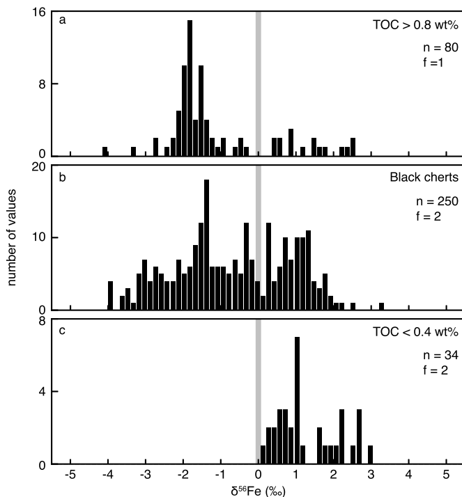
Fig. 7. Pyrite \delta^{56}\text{Fe} distributions in cherts with variable total organic carbon (TOC) content. Experimental works suggested that organic matter could catalyze pyrite formation by providing active surfaces for pyrite nucleation (Rickard et al., 2007; Rickard, 2012; Duverger et al., 2021). The upper plot (a) comprises pyrite \delta^{56}\text{Fe} values from cherts containing 0.82 to 1.51 wt% organic carbon. The middle plot (b) includes \delta^{56}\text{Fe} values measured in black cherts for which no specific information about the organic carbon content was given. We suggest that they can reasonably be considered as organic matter-rich host rocks. In the lower plot (c), \delta^{56}\text{Fe} values were measured in pyrites associated with cherts presenting TOC values from less than 0.05 to 0.38 wt%. The numbers of values (n) and geological formations (f) from which pyrite originates are indicated. Pyrite particles in organic matter-poor and organic matter-rich (TOC > 0.8 wt%) cherts have one location in common (Mendon Formation). The three other locations are distinct. The grey bar represents a \delta^{56}\text{Fe} value of 0‰ and is drawn to facilitate comparison between plots.
