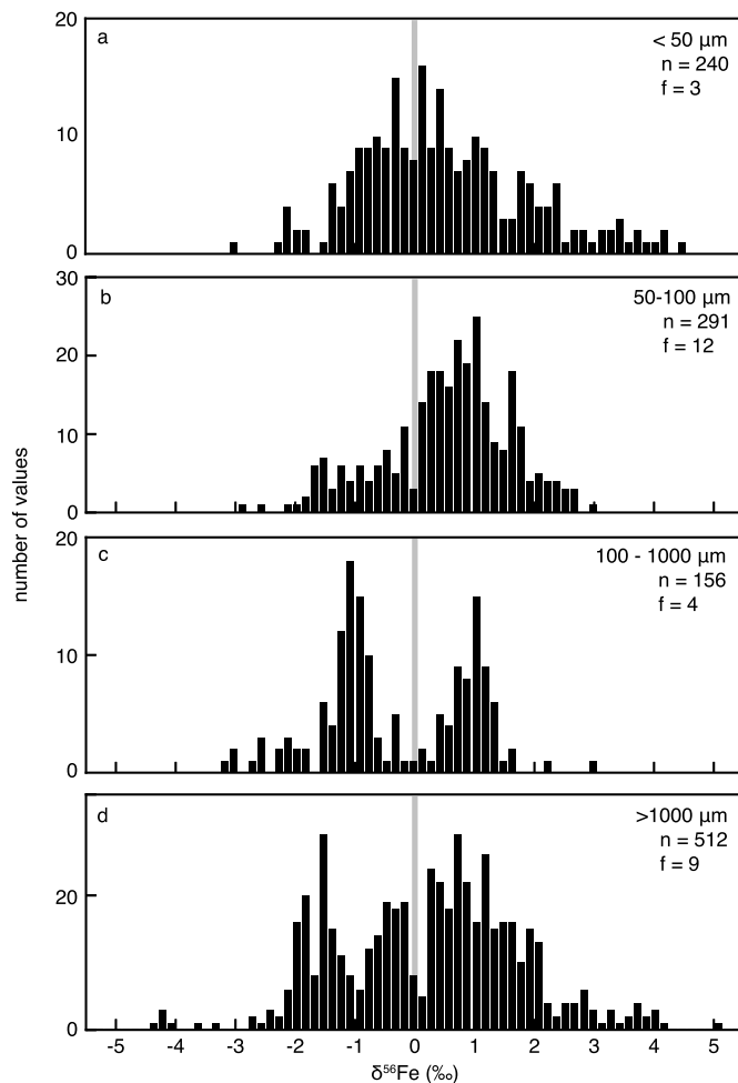
Fig. 3. Pyrite \delta^{56}\text{Fe} distributions as a function of pyrite grain size. Four groups are differentiated: (a) grains with size <50 \mu\text{m} , (b) grains with size comprised between 50 and 100 \mu\text{m} , (c) grains with size of a few hundreds of microns, and (d) millimeter grains. Information on pyrite grain size was not systematically available in previous publications. Further detail on grains with size comprised between 100 and 1000 \mu\text{m} was not always available. The numbers of values (n) and geological formations (f) are indicated for each histogram. The vertical grey bar represents a \delta^{56}\text{Fe} value of 0‰ and is drawn to facilitate comparison between plots.
