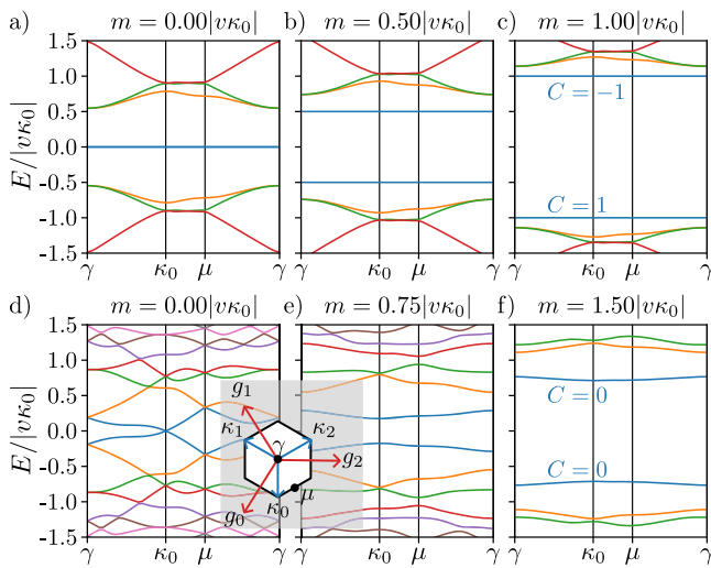
Fig. 1 | Band structure in the two sole massive chiral limits of C_3 symmetric moiré material with Dirac cones in presence of an additional mass m . The first (a–c) and second (d–f) chiral limits reproduce those of TBG when m = 0 (a, d) and feature isolated narrow bands for large values of the mass (c, f). Exact flat bands with opposite Chern numbers appear in the first chiral limit (a–c) for any m due to a chiral anomaly with non-zero Atiyah–Singer index—analogueous to the zeroth Landau level of graphene in presence of sublattice potential difference. We used \alpha = \alpha_c in (a–c, see Eq. (3)), \alpha = 1.2\alpha_c and r = 0 in (d–f, see Eq. (4)), and the inset shows high symmetry points in reciprocal space, with g_n = \kappa_n - \kappa_{n-1} .
