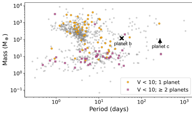
Figure 14. Planet mass vs. planet orbital period for all systems with masses measured to 30% or better uncertainty. We have highlighted planets around bright stars in color. Within the bright star sample, we distinguish between single-planet systems (orange circles) and systems with more than one planet (purple squares). TOI 4633 c is the second longest-period planet in a bright host star system (however, we do note that planet c does not have a mass measured to 30% or better uncertainty). Furthermore, both planets in the system are fairly high mass and likely not rocky, which is unusual compared to the confirmed population of multi-planet systems.
