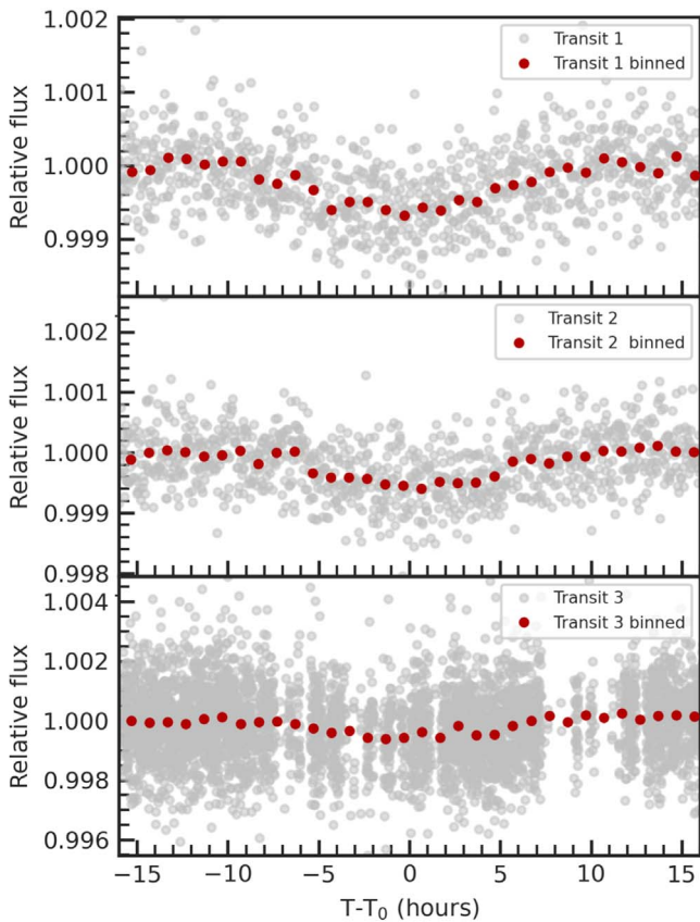
Figure 2. The three transits of TOI 4633 c. Nominal TESS observations are shown in light gray while solid circles represent 60 minutes binned data.
