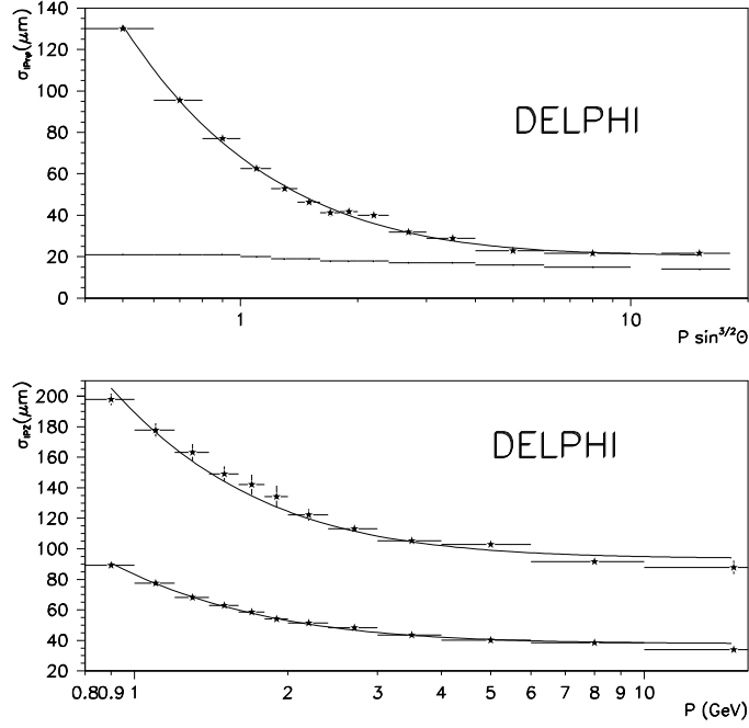
Figure 13: Upper: Mean track extrapolation uncertainty in R\phi measured as a function of p \sin^{3/2} \theta ( p in \text{GeV}/c ). The values are determined by subtracting quadratically the vertex position uncertainty, shown by the bottom curve, from the measured impact parameter uncertainty. The full line depicts (65/p \sin^{3/2} \theta \oplus 20) \mu\text{m} . Lower: Mean track extrapolation uncertainty in the Rz plane, measured similarly as a function of the particle momentum. The two curves correspond to tracks with 80^\circ < \theta < 90^\circ (bottom) and 45^\circ < \theta < 55^\circ (top). The full lines depict (71/p \oplus 39) \mu\text{m} and (151/p \oplus 96) \mu\text{m} respectively.
