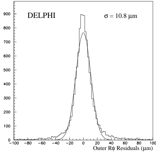
Figure 6: Vertex detector residual distribution in the R\phi plane from tracks passing through the overlap regions in the Outer layer.
