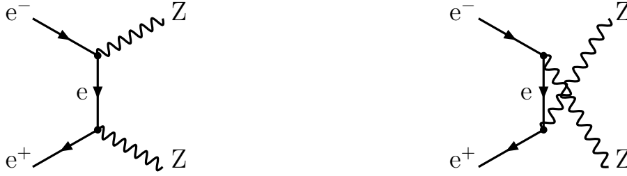
Figure 1: The Feynman graphs for on-shell ZZ production (referred to as the NC02 graphs)
