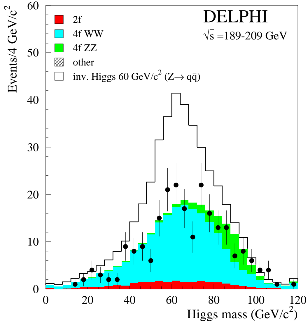
Figure 9: Hadronic channel low mass analysis: Reconstructed Higgs boson mass for \sqrt{s} from 189 to 209 GeV after the final selection. The white histogram corresponds to a Higgs boson with 60 \text{GeV}/c^2 mass decaying with a branching fraction of 100% into invisible modes.
