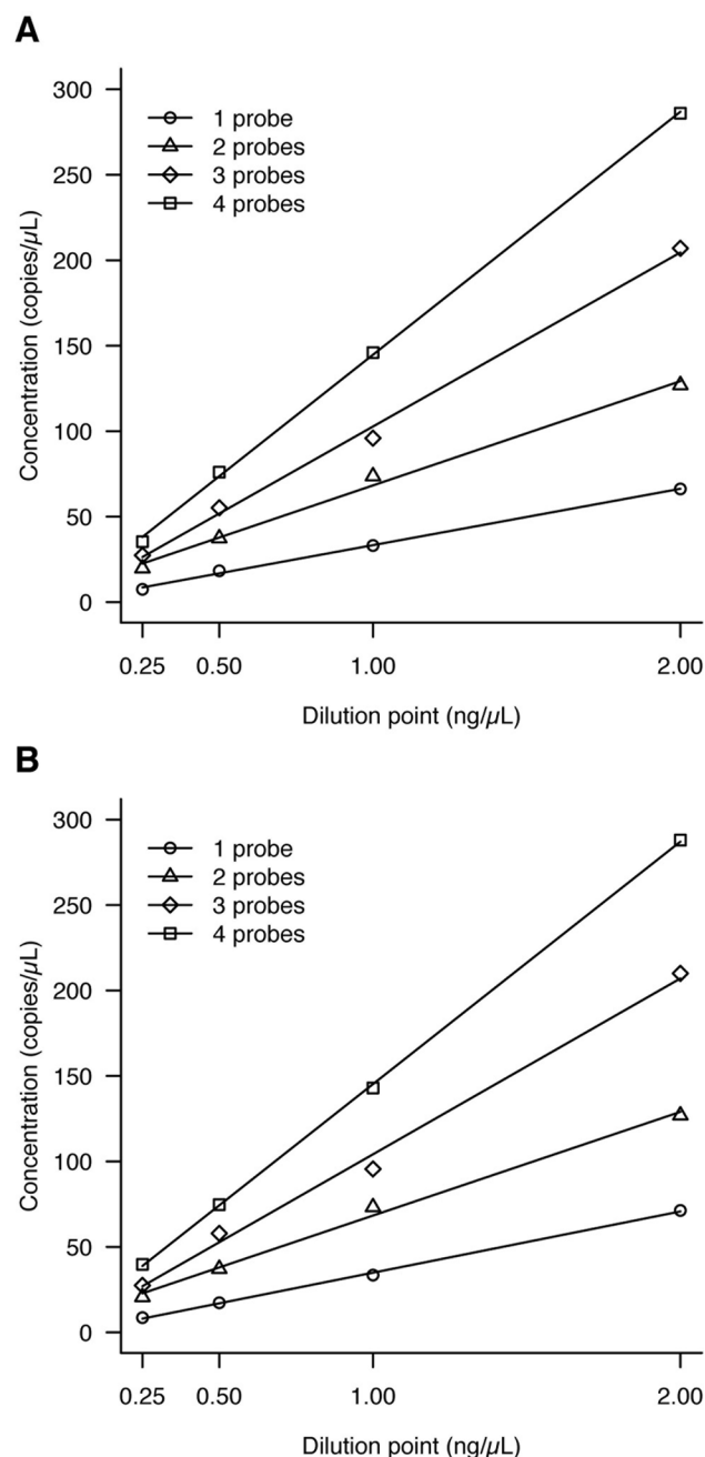
Fig 1. Validation of the multiplex PCR–serial dilutions for each set of probes. A: FAM probes (chromosome 21), B: VIC probes (reference chromosome).
