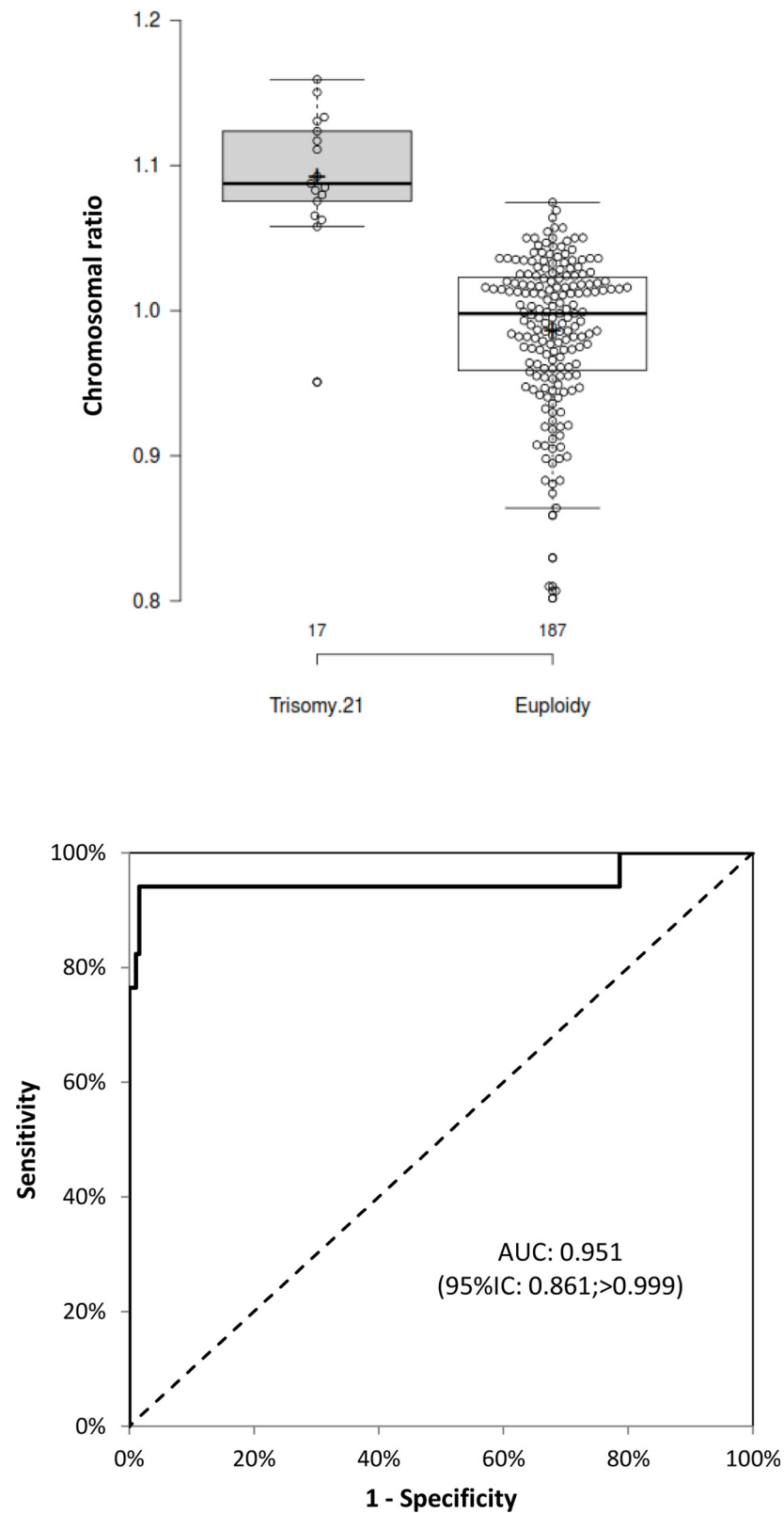
Fig 3. Box-and-whisker/Beeswarm plots of the distribution of chromosome ratios in the two groups (upper plot), and the ROC curve for the chromosome ratio as a predictor of trisomy 21 (lower plot) for samples exceeding the threshold for the number of positive PCRs. In the upper plot, the box displays the
