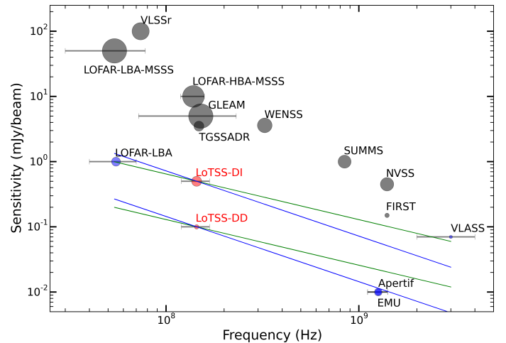
Fig. 1. A summary of the sensitivity, frequency and resolution of a selection of recent and planned large-area radio surveys (see also Table 1). The size of the markers is proportional to the square root of the survey resolution. Grey, blue and red markers show the ongoing/completed surveys, forthcoming surveys, and the LOFAR HBA surveys respectively. The horizontal lines show the frequency coverage for surveys with large fractional bandwidths ( > 0.2 ). The green sloping lines show the sensitivity that is equivalent to that achieved in the LoTSS direction-dependent (DD) calibrated and direction-independent (DI) images for typical radio sources with a spectral index \sim -0.7 . Similarly, the blue sloping lines show the equivalent sensitivity to steep spectrum sources with a spectral index \sim -1.0 .
