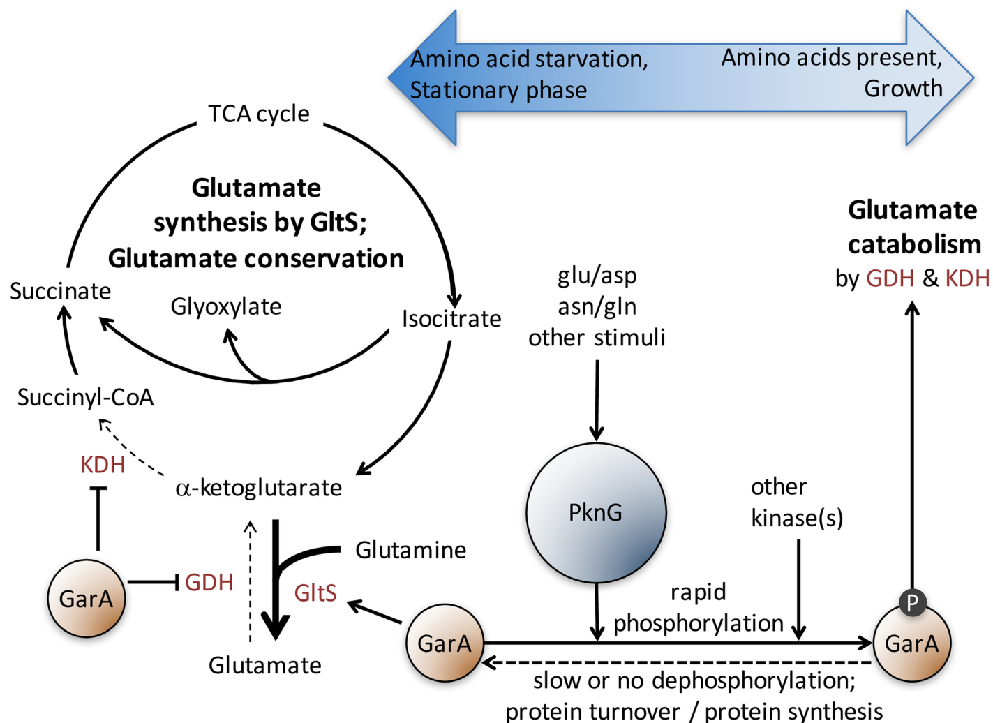
Fig 8. A model depicting control of the TCA cycle and glutamate metabolism by PknG and GarA. When PknG activity is low, unphosphorylated GarA activates glutamate synthesis and inhibits glutamate catabolism by direct binding to the relevant enzymes. When PknG activity is stimulated, for example by glutamate and aspartate, GarA become phosphorylated, causing a shift in metabolism towards glutamate catabolism. KDH is the alpha-ketoglutarate dehydrogenase complex, GDH is glutamate dehydrogenase, GltS is glutamate synthase.
