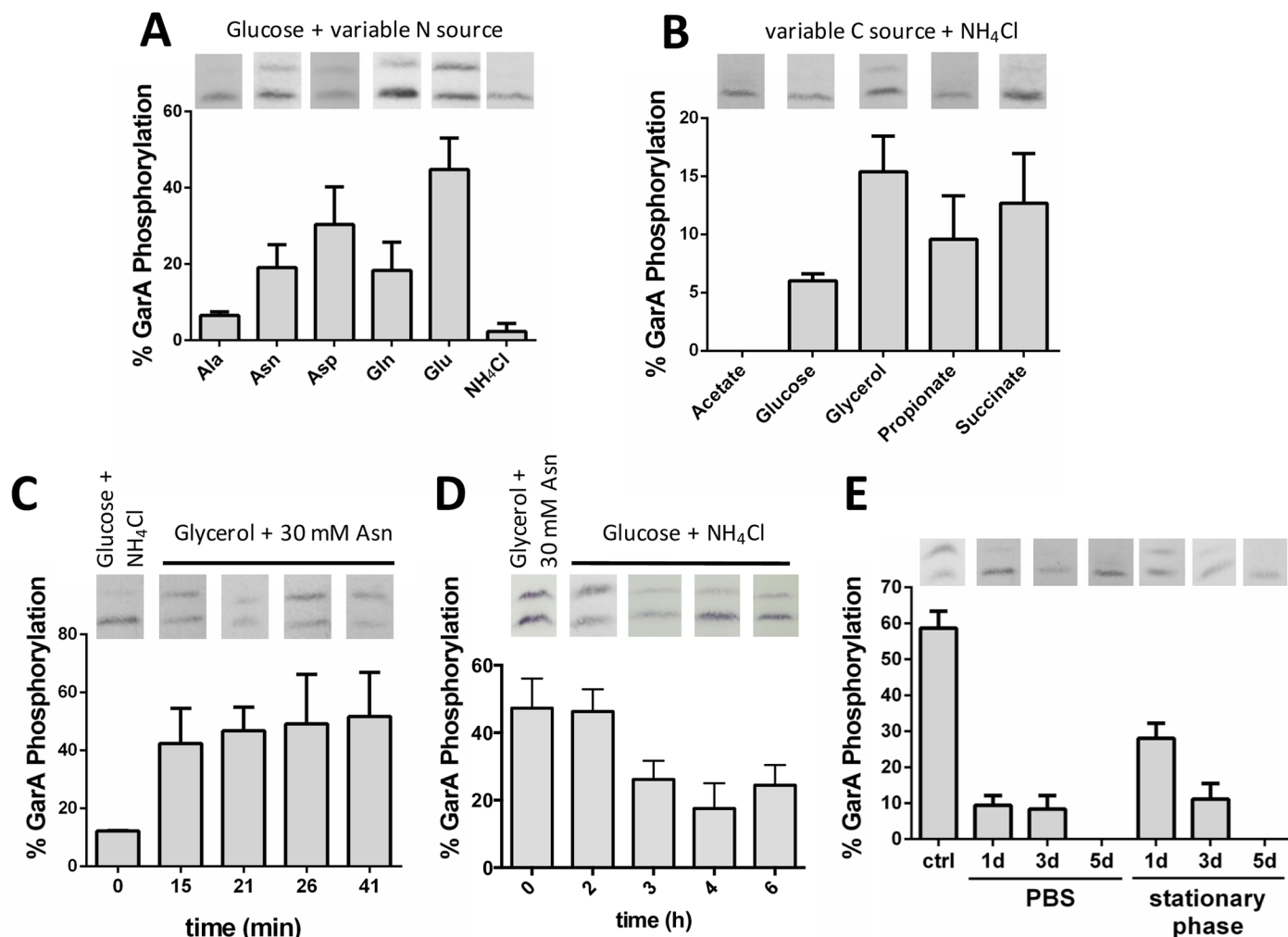
Fig 5. GarA phosphorylation in M. smegmatis was regulated by nutrient availability. The reporter strain of M. smegmatis was cultured in different media and cell lysates analysed by Western blot and densitometry. (A) Glutamate and related amino acids triggered phosphorylation of GarA: the nitrogen source is indicated and the carbon source was glucose. (B) The supplied carbon source affected phosphorylation of GarA: the carbon source is indicated and the nitrogen source was NH 4 Cl. (C) Phosphorylation of GarA occurred rapidly when cells were cultured in poor medium and then given supplementary nutrients (initially 1% glucose with 10 mM NH 4 Cl and 0.05% tyloxapol, then 1% v/v glycerol and 30 mM asparagine were added at time zero). (D) Dephosphorylation of GarA occurred slowly when cells switched from rich to poor medium (initially 1% glycerol with 30 mM asparagine and 0.05% Tween 80 then switched to 1% glucose with 10 mM NH 4 Cl and 0.05% tyloxapol). (E) GarA was predominantly unphosphorylated when M. smegmatis were in stationary phase or starved in PBS. The reporter strain of M. smegmatis was grown in Sauton's medium with shaking for 5 days. For the starvation experiment exponentially growing M. smegmatis were washed with PBS and incubated in PBS with 0.05% tyloxapol for 5 days. Values represent mean and standard deviation of at least three independent replicates.
